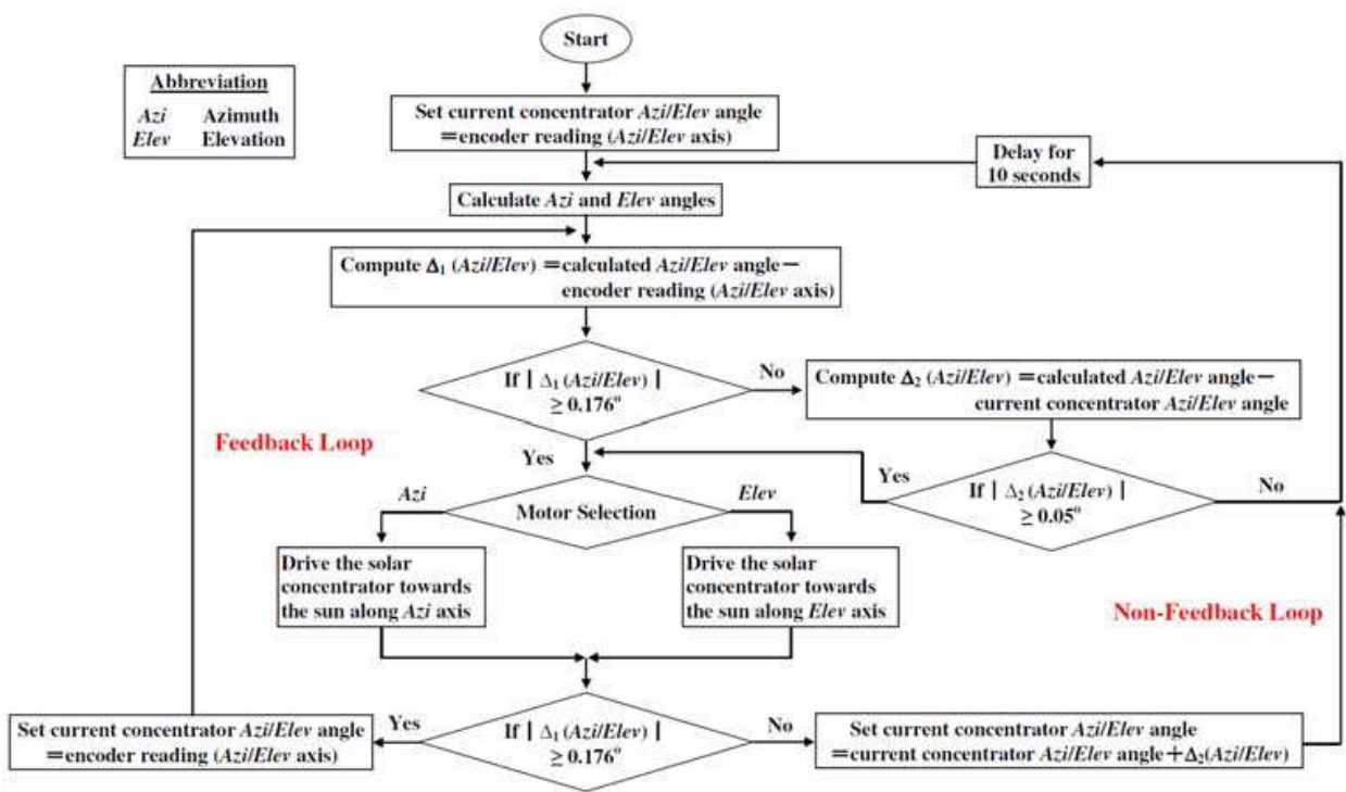
Fig. 16. The algorithm flow of the sun-tracking control program that including motor step count, 1.64 \times 10^{-4} \text{ }^\circ/\text{step} , in fine-tuning the position of solar concentrator prototype and improving the sun tracking accuracy beyond the resolution of the optical encoder.
