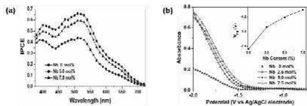
Fig. 13. (a) Action spectra of the dye-sensitized solar cells based on the undoped and Nb-doped TiO 2 electrodes. (b) Optical absorbance at 870 nm of undoped and Nb-doped TiO 2 films measured as a function of applied potential. Inset shows the flat-band potential of the samples as a function of the Nb contents
