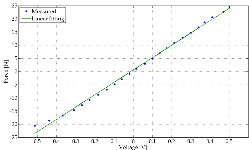
Fig. 9. Calibration curve with broadband demodulation.
