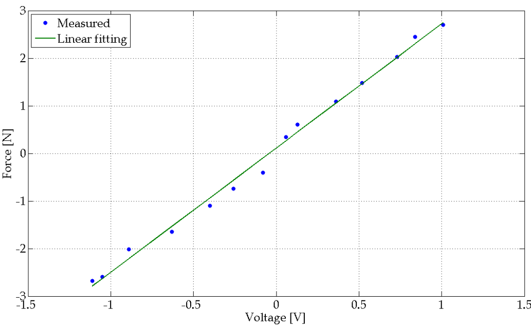
Fig. 8. Calibration curve with narrow band demodulation.
