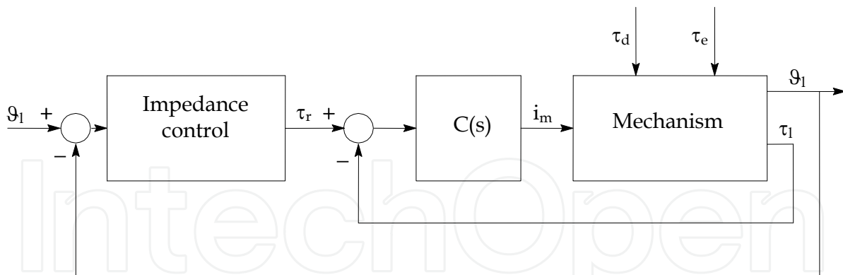
Fig. 12. Compliance control scheme.
