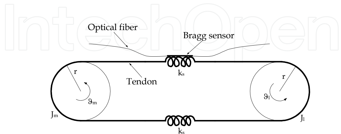
Fig. 11. Sketch of the test bench.
