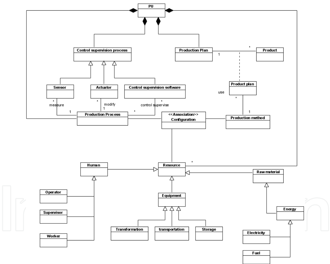
Fig. 3. Holonic Production Unit (From (Chac3n et al., 2008))
