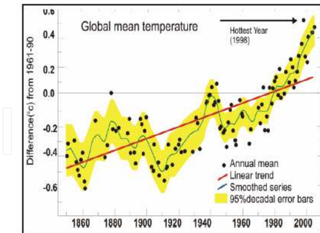
Fig. 1. Global mean temperature anomalies, 1860-2005 (IPCC 2007)
