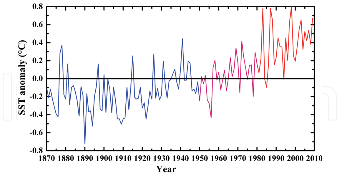
Fig. 1. SST anomaly over the NIO ( 40^{\circ}\text{E} - 100^{\circ}\text{E} , 5^{\circ}\text{N} - 25^{\circ}\text{N} ) during southwest monsoon season. Blue, pink and red colour indicates 1870 – 1949, 1950 – 1980 and 1981 – 2009 respectively.
