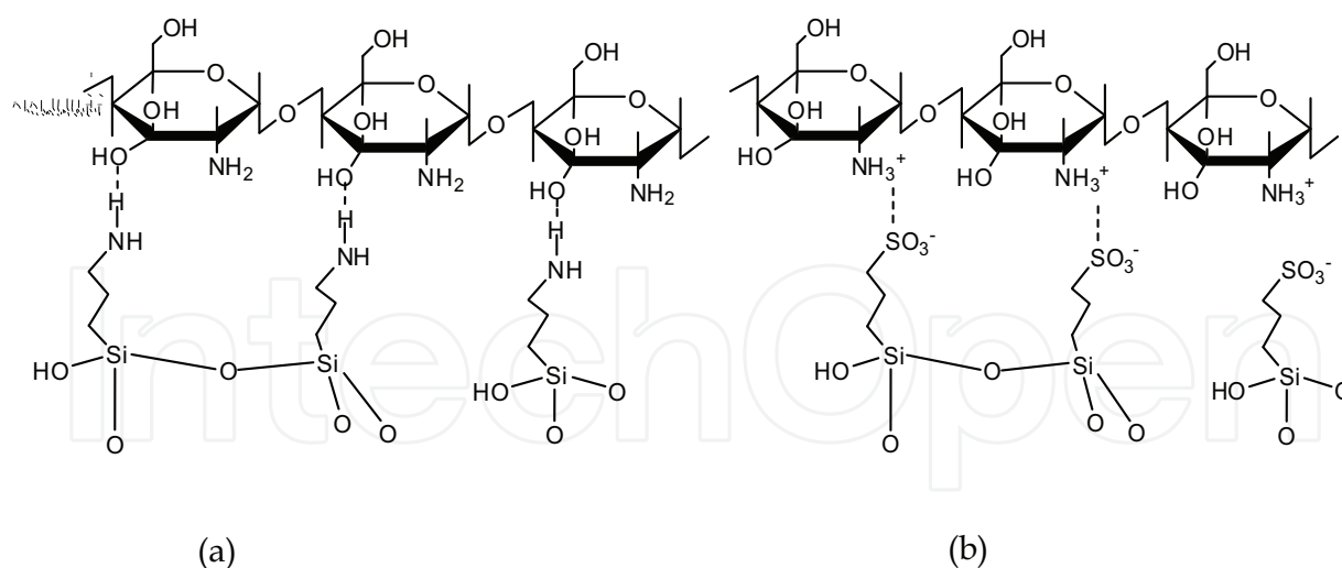
Fig. 6. Schematic presentation of interfacial interaction between modified-zeolite-filled chitosan membranes (a) CS- \text{H}_2\text{NY} membranes and (b) CS- \text{HO}_3\text{SY} membranes
