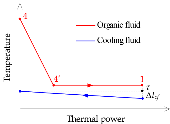
Fig. 16. Condenser heat exchange diagram
