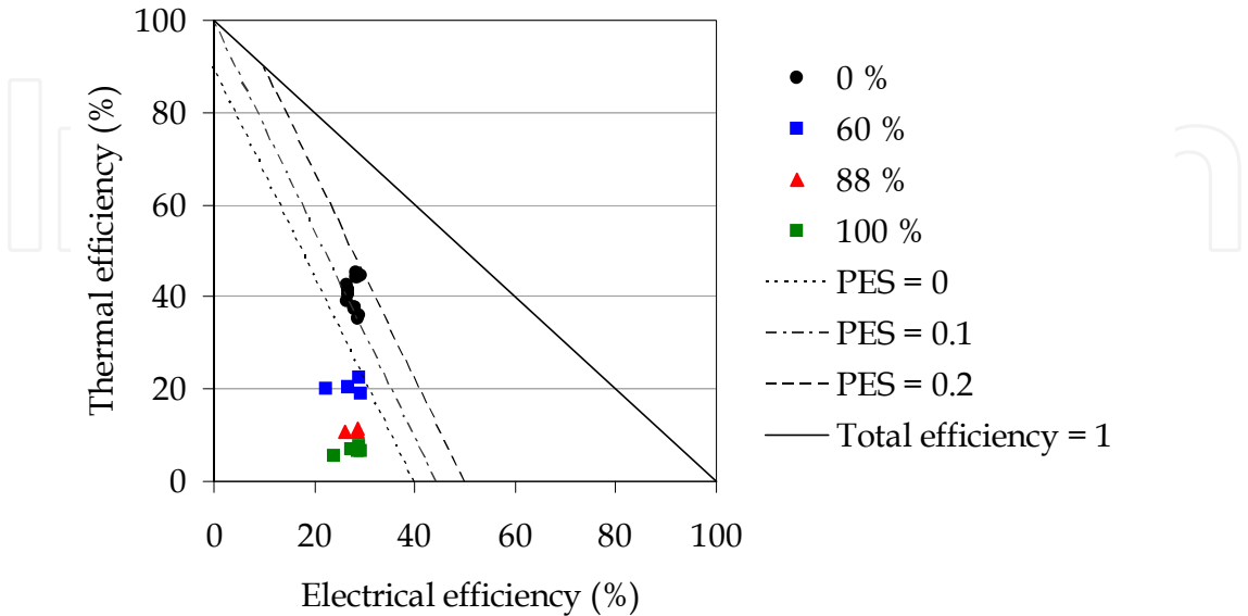
Fig. 9. PES for different degrees of BPV opening
