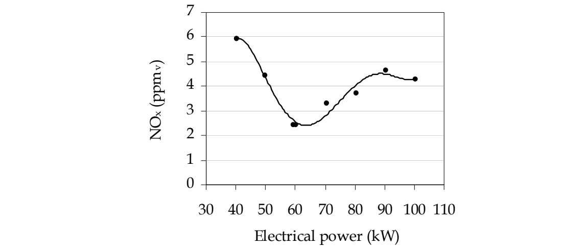
Fig. 7. NO x concentration @ 15 % O 2
