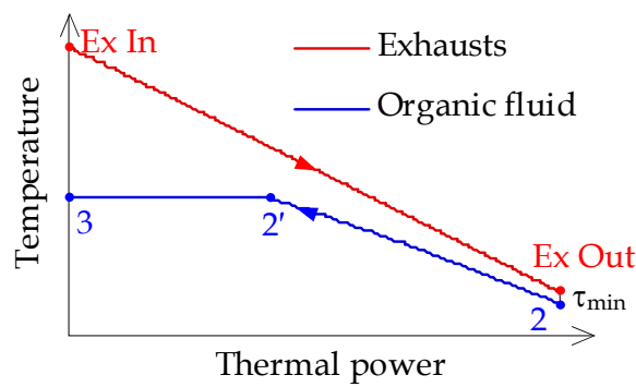
Fig. 17. Rankine cycle heat exchange diagram
