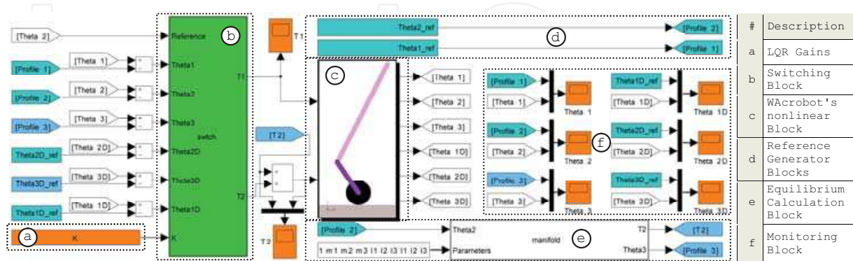
Fig. 11. The Simulink ® block diagram of the WAcrobot system with tracking controller The WAcrobot system with gain scheduling tracking controller simulated in Simulink ® is illustrated in Figure 11. Figure 12 shows the simulation results of the wheels and arm tracking task. In this figure the simulation responses of the angular positions and velocities
