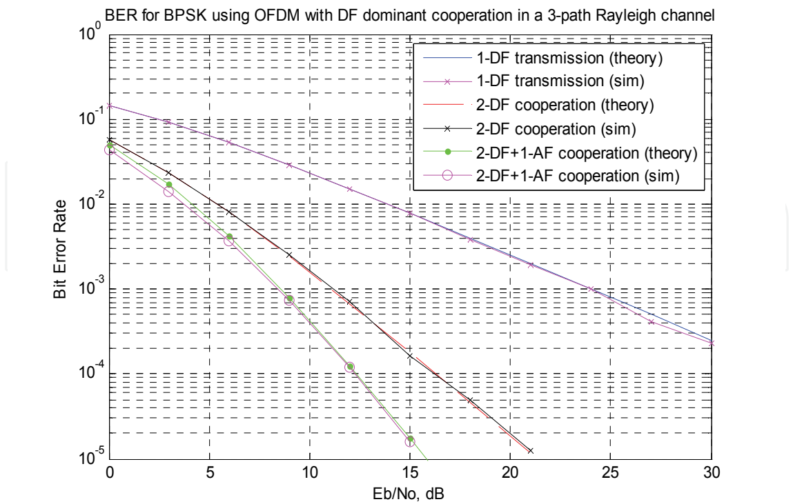
Fig. 10. BER performance for DF dominant OFDM cooperation.
