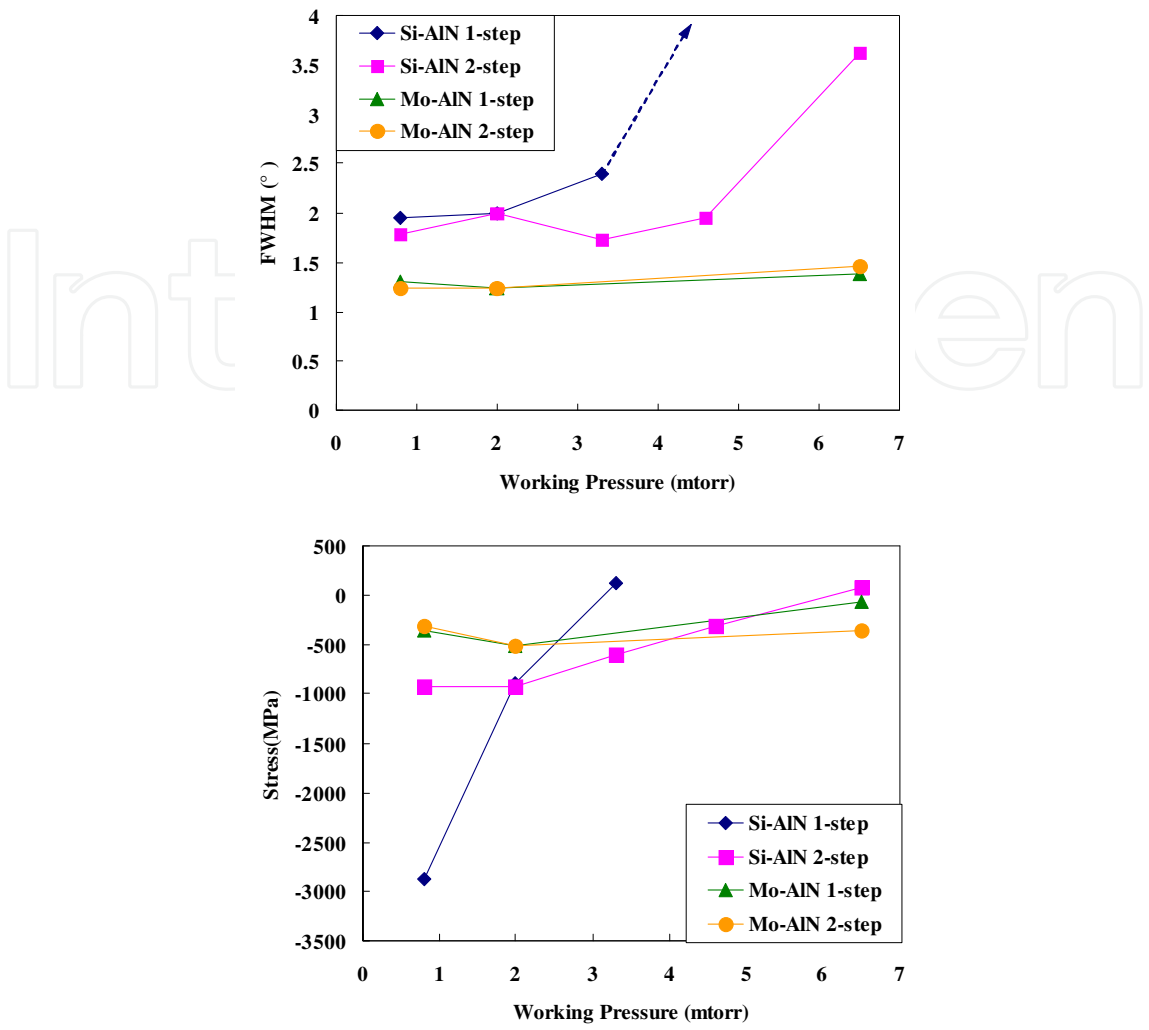
Fig. 7. Effects of working pressure on (a) XRD FWHM, and (b) residual stress of AlN piezoelectric layer for both one-step and two-step sputtering, respectively [Cherng et al 2008]
