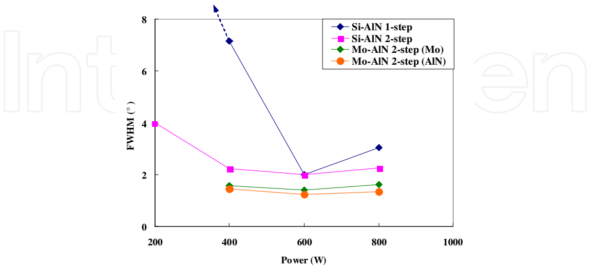
Fig. 8. Effects of discharge power on XRD FWHM for both one-step and two-step sputtering [Cherng et al 2009].
