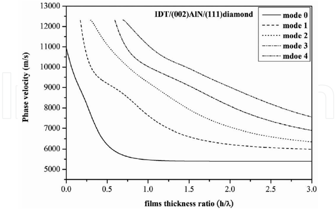
Fig. 12. Phase velocities dispersion curves of the first five Rayleigh SAW modes propagation in the IDT/(002)AlN/(111)diamond [Wu et al 2008].
