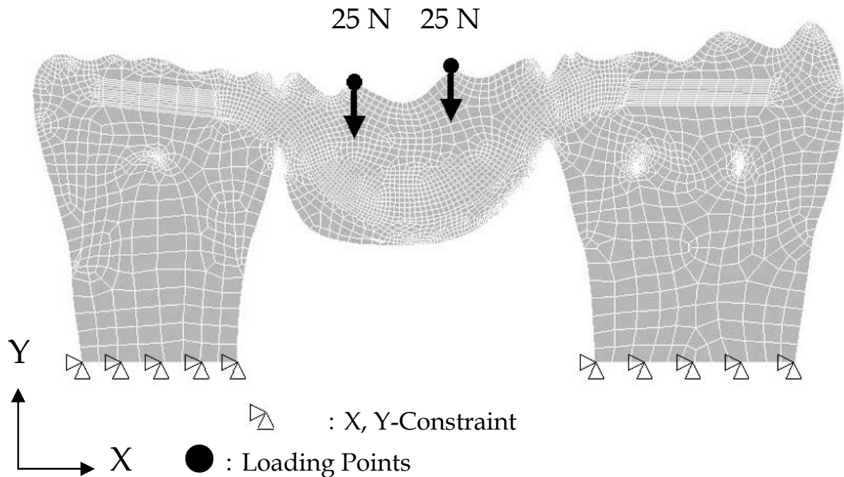
Fig. 25. Boundary conditions of finite element models (GFR1.0)
