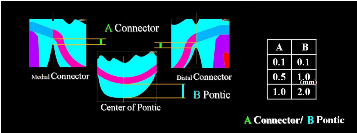
Fig. 15. The position of the fiber framework
