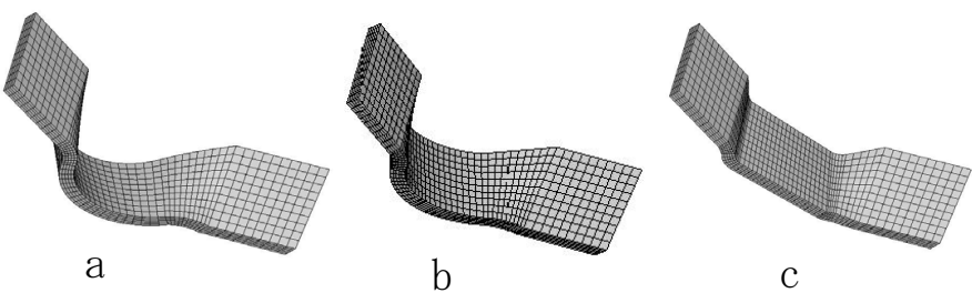
Fig. 6. Three different glass fiber framework a: FRC1 labial side, curved line b: FRC2 at the center, curved line c: FRC3 lingual side, straight line
