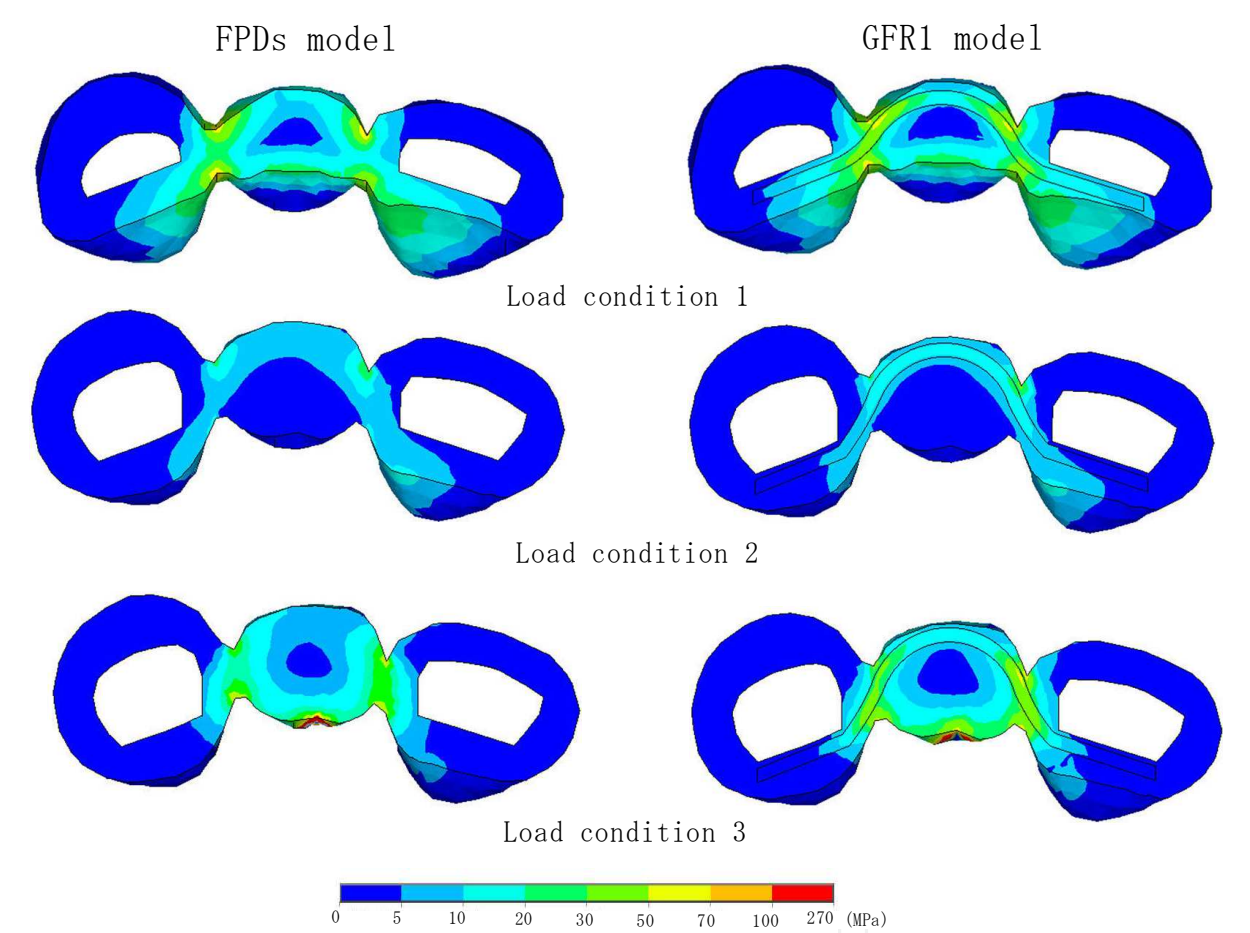
Fig. 13. Maximum principal stress at the horizontal cross section. A = C-FPD; B = FRC1.
