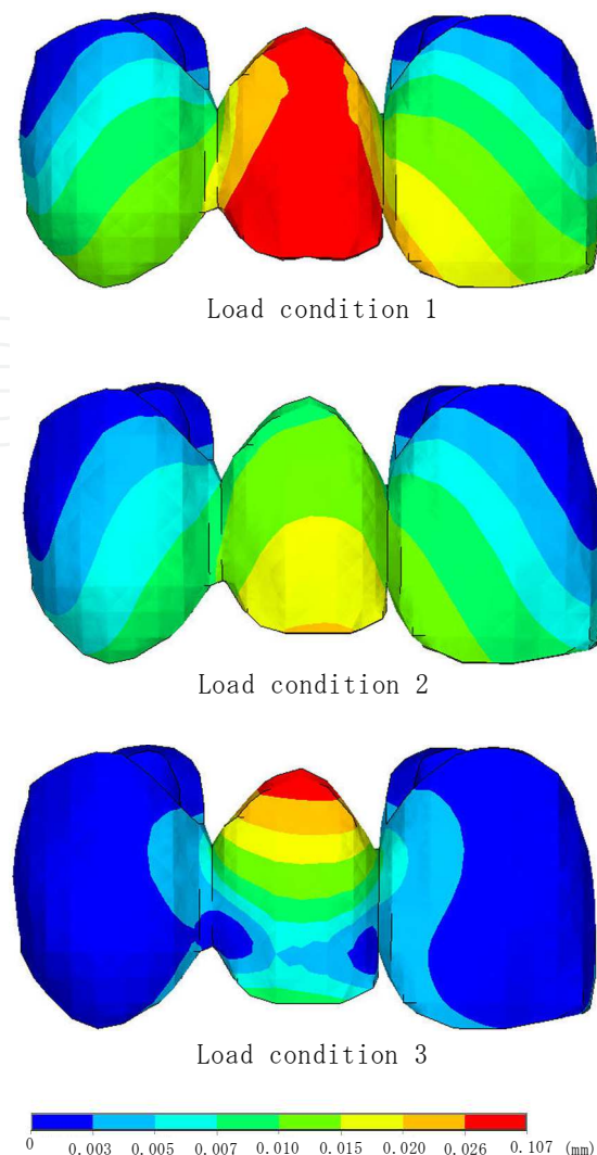
Fig. 10. Displacement distributions of FPDs(Labial view)
