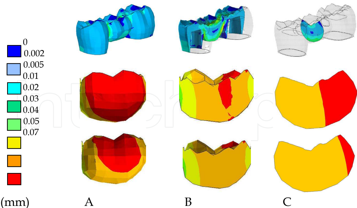
Fig. 33. Displacement of the pontic against vertical load Upper: C-FPD. Lower: FRC-FPD A; Surface view of buccal side. B; Mesiodistal section. C; Buccolingual section
