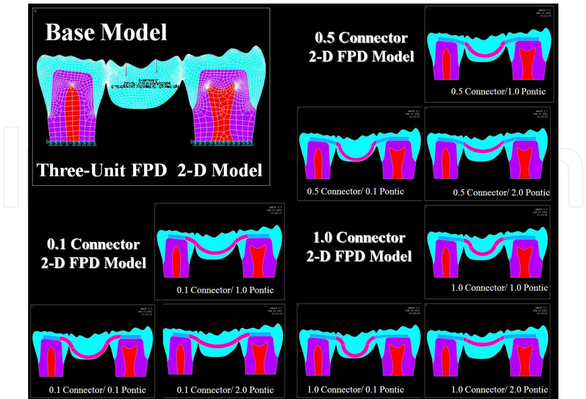
Fig. 16. Nine different 2-D FE FRC hybrid composite FPD models.
