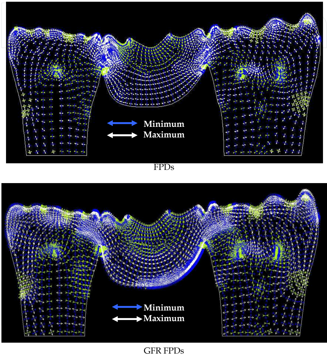
Fig. 27. Depiction of stress vector
