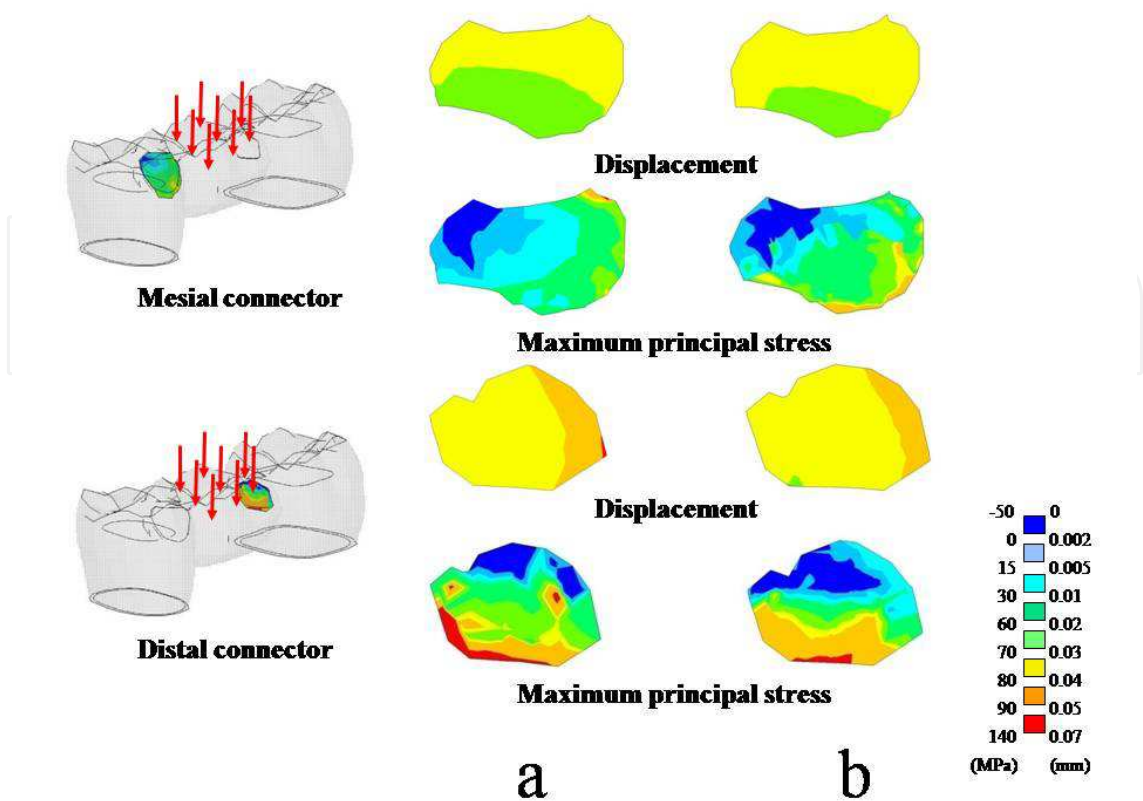
Fig. 39. Vertical load at buccolingul cross section of mesial and distal connector a: C-FPD. b: FRC-FPD
