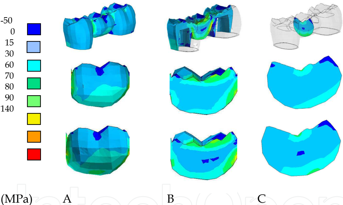
Fig. 34. Maximum principal stress of the pontic against lateral load Upper: C-FPD. Lower: FRC-FPD A; Surface view of buccal side. B; Mesiodistal section. C; Buccolingual section
