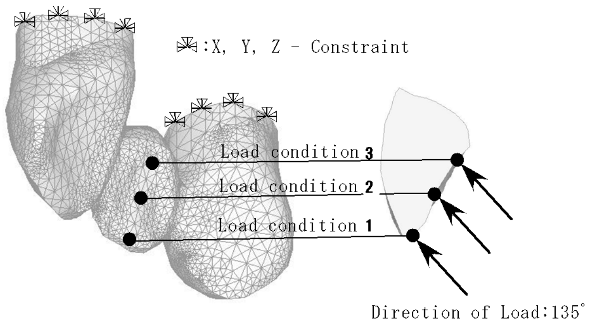
Fig. 8. Boundary conditions.
