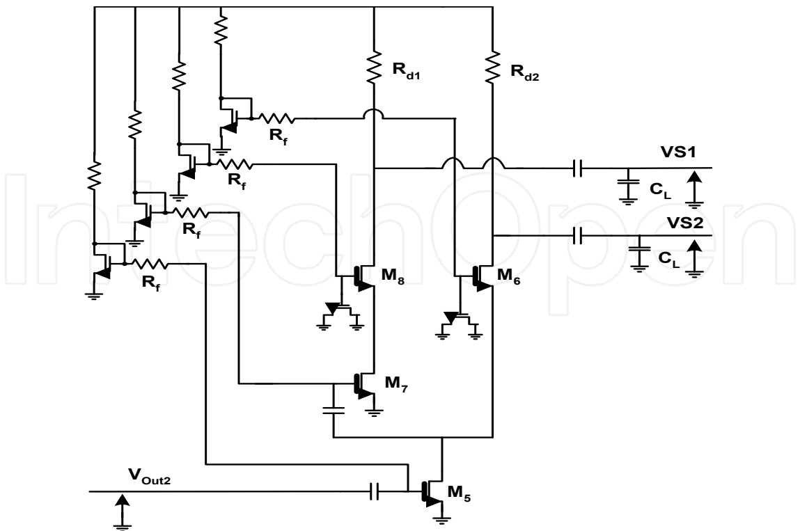
Fig. 9. Single ended to differential ended conversion stage.
