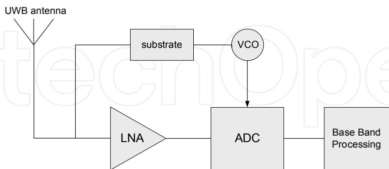
Fig. 13. Typical IR-UWB receiver architecture
