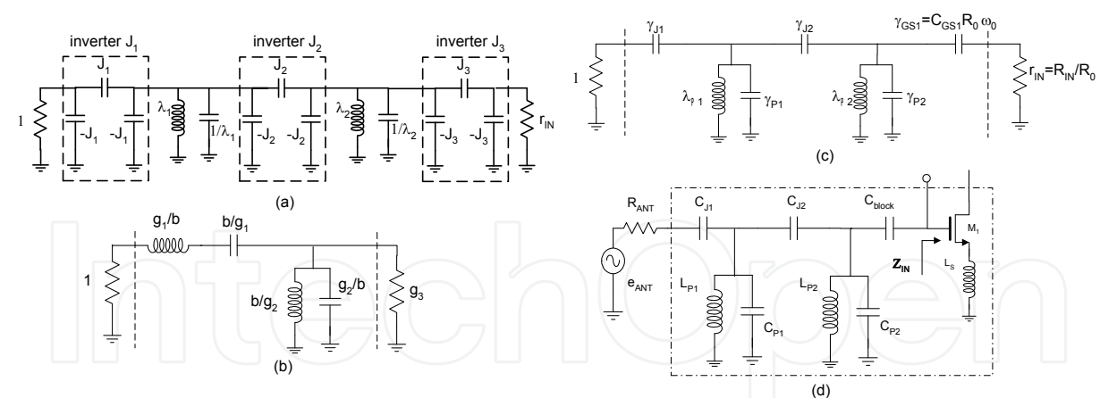
Fig. 3. Single ended broadband input matching cell for small fractional bandwidths. (a) Input matching cell architecture showing the admittance inverters. (b) Equivalent LC ladder filter (c) Input matching cell equivalent circuit. (d) LNA broadband input matching cell architecture.
