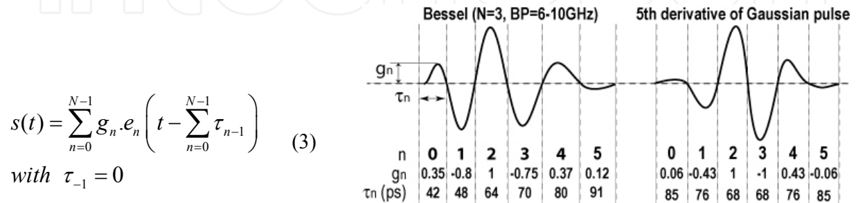
Fig. 3. Principle of synthesis by pulse combination.
