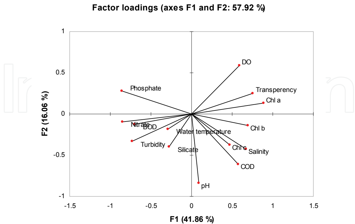
Fig. 4. Factor loading plot of the water quality parameters
