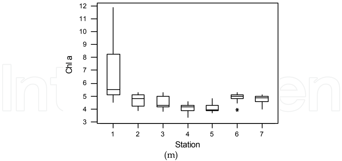
Fig. 2(m). Box plot diagrams of the 14 water quality parameters form coastal waters of Sundarban wetland
