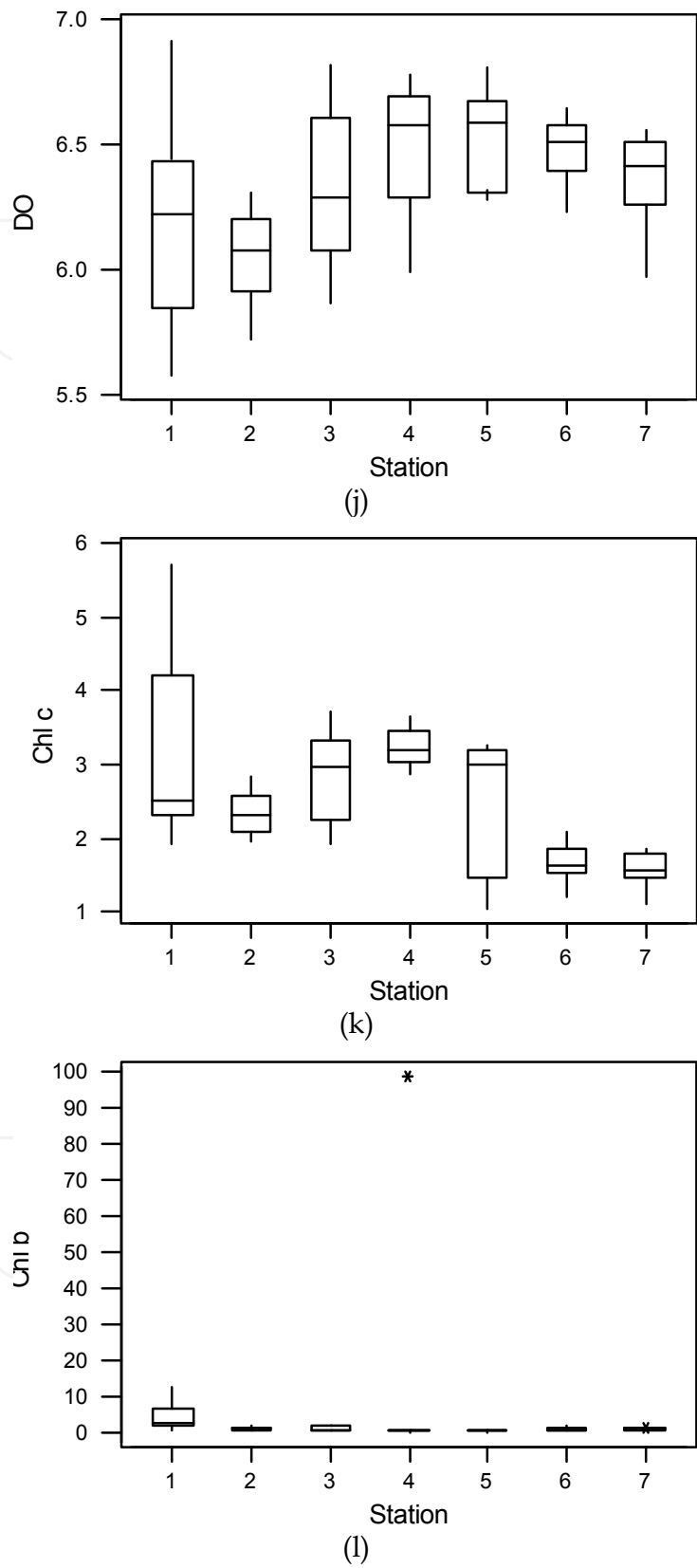
Fig. 2(i-l). Box plot diagrams of the 14 water quality parameters form coastal waters of Sundarban wetland
