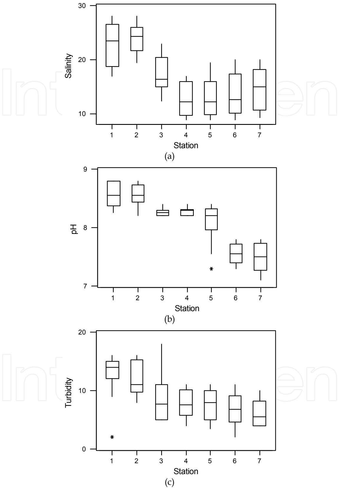
Fig. 2(a-c). Box plot diagrams of the 14 water quality parameters form coastal waters of Sundarban wetland
