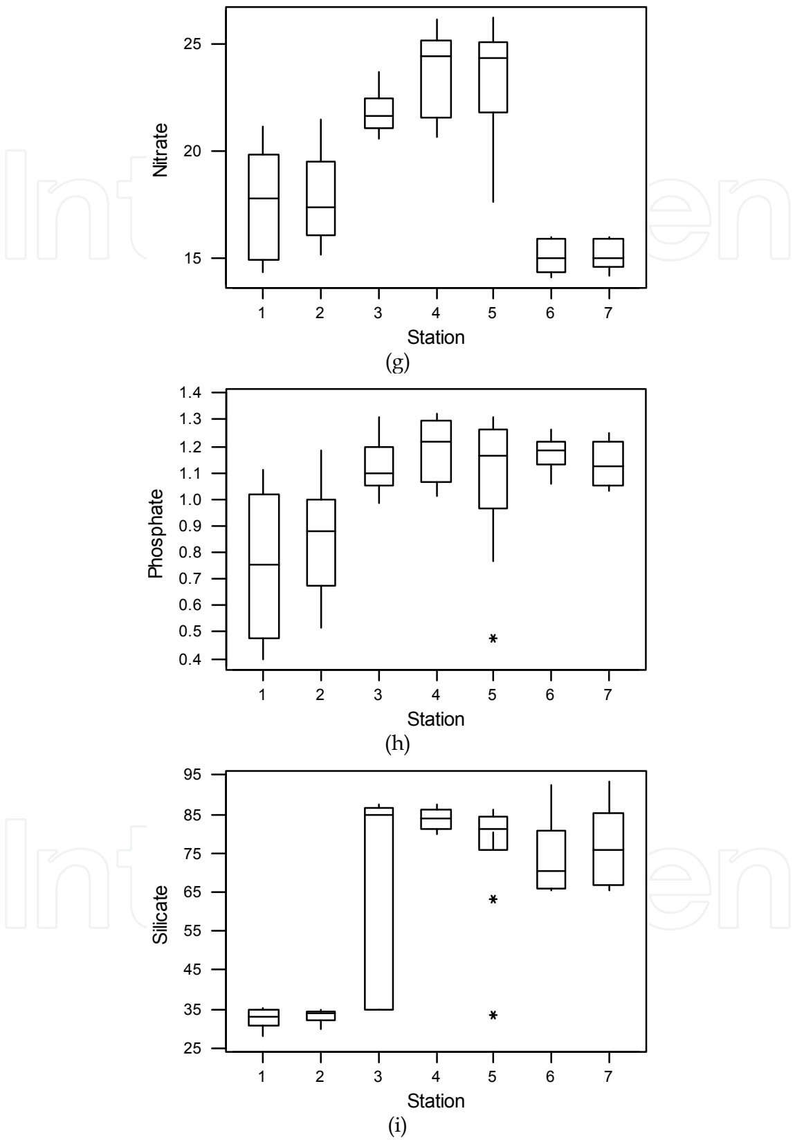
Fig. 2(g-i). Box plot diagrams of the 14 water quality parameters form coastal waters of Sundarban wetland
