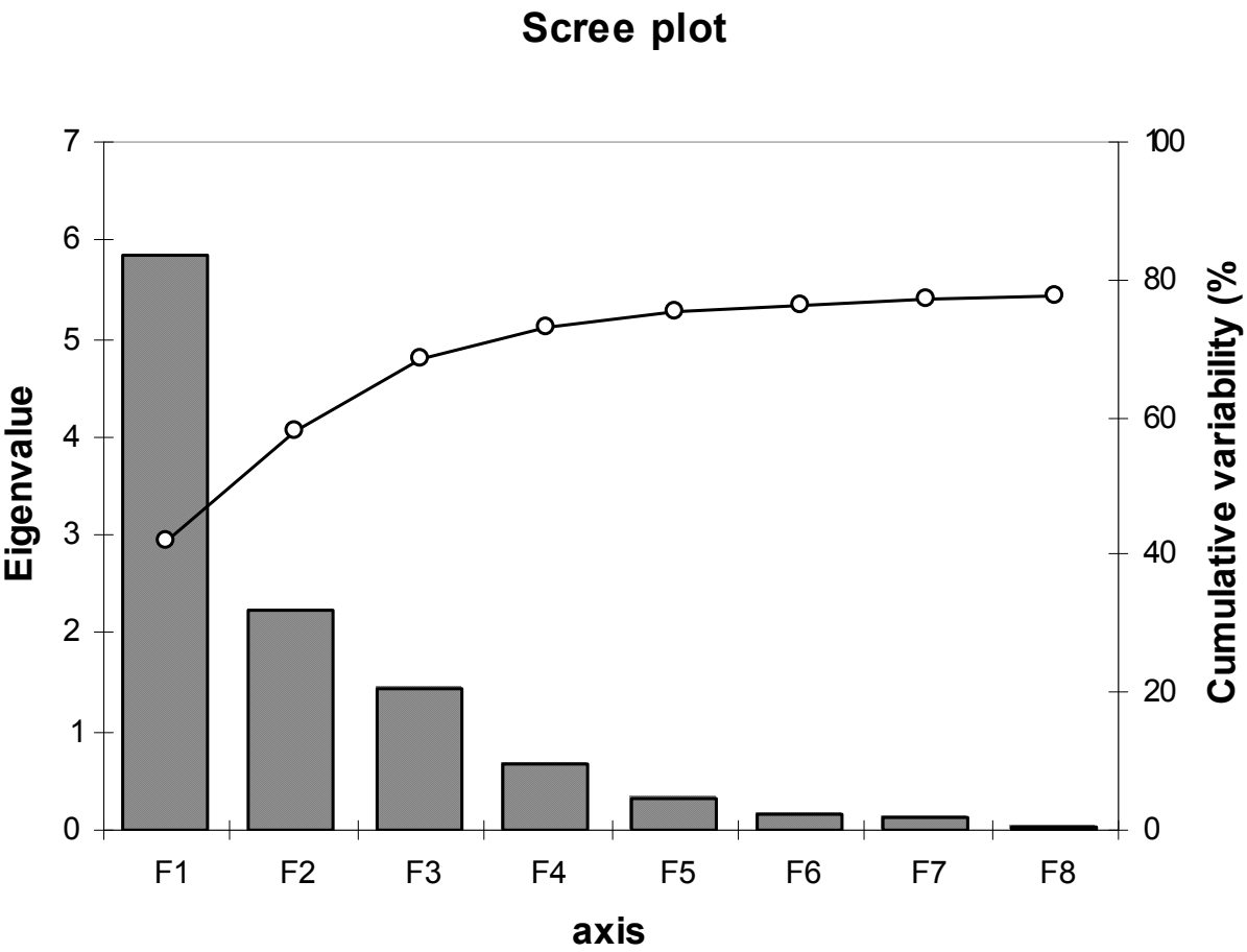
Fig. 3. Scree plot of the factor analysis after varimax rotation
