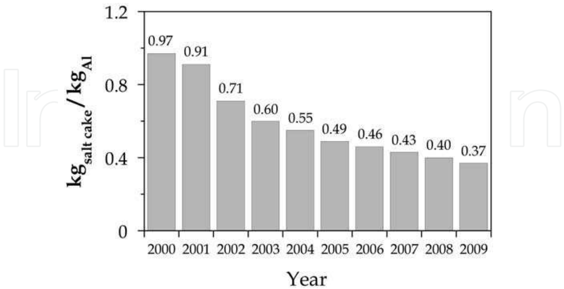
Fig. 4. Evolution of the salt cake generated with respect to the aluminium recovery obtained.
