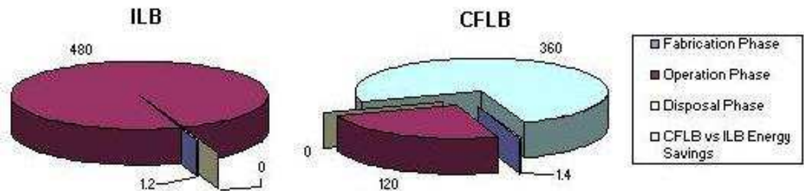
Fig. 1. Life-Cycle Energy of ILBs vs CFLBs (units in kWh).
