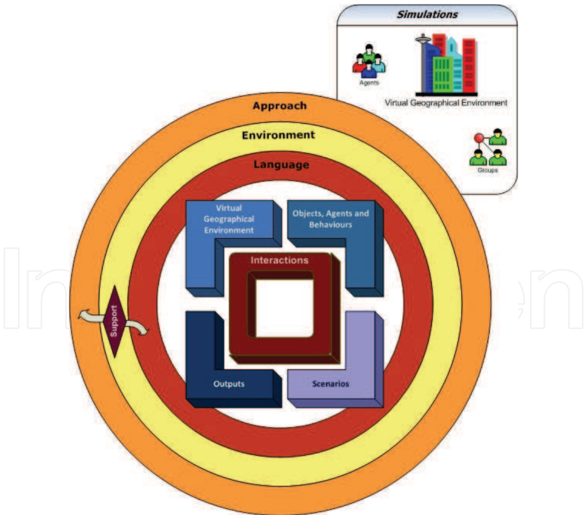
Fig. 3. PLAMAGS' architecture.
