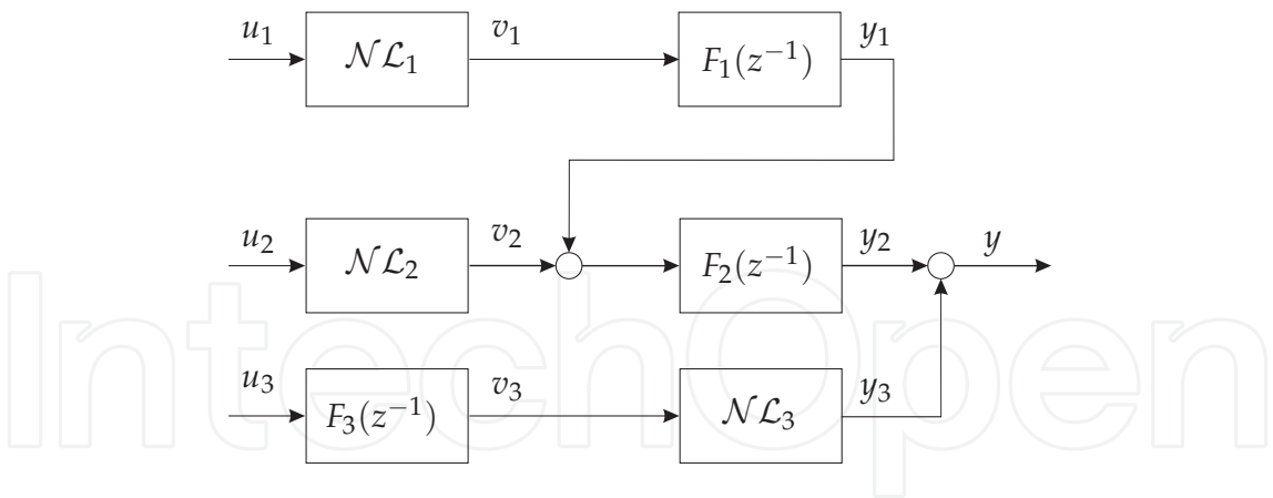
Fig. 9. Structure of the nonlinear MISO model
