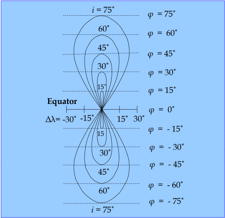
Fig. 39. Graphical illustration of apparent orbits of relative motion of 24-hour satellites on their circular orbit for different inclinations of their orbits, as a spectator on the Earth sees them.
