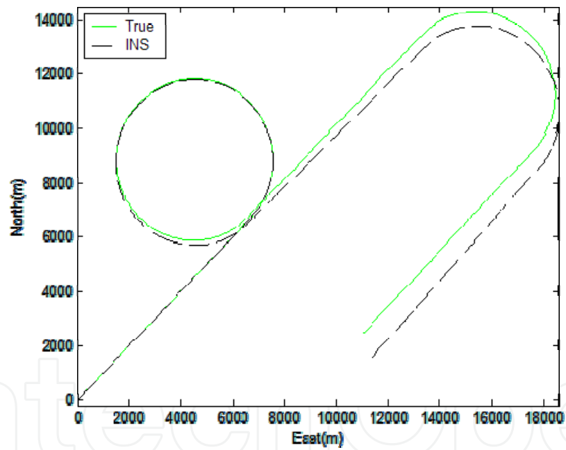
Fig. 11. Trajectory for the simulated vehicle (solid) and the INS derived position (dashed)
