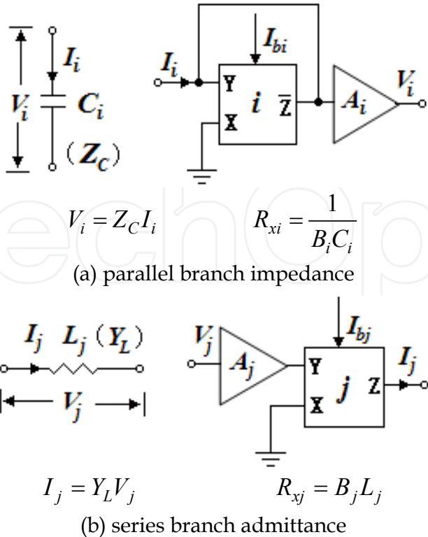
Fig. 6. Partial branch simulations using OA and CCCII of the lowpass network of Fig. 5
