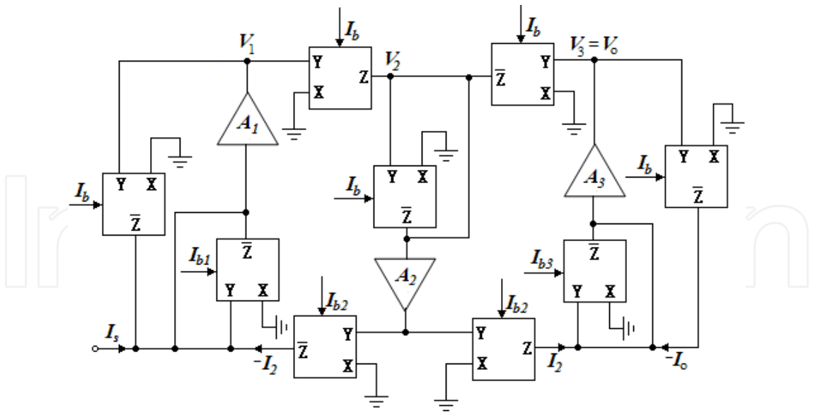
Fig. 7. Systematic diagram for current-mode 3rd-order lowpass filter using active-only elements
