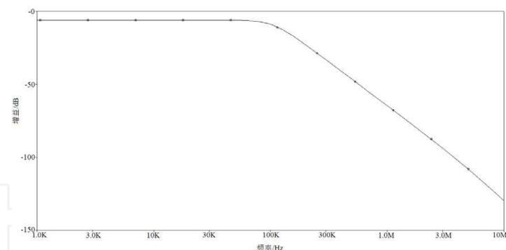
Fig. 11. Simulated frequency response of Fig. 7
