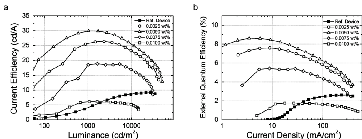
Fig. 5. Current efficiency ( \eta_c ) vs. luminance (a) and external quantum efficiency ( \eta_{ext} ) vs. current density (b) of the single-layered Ir(ppy) 3 sample devices (open symbols) with various concentrations of Bu 4 NBF 4 and reference device (closed square). (Oh et al., 2007)
