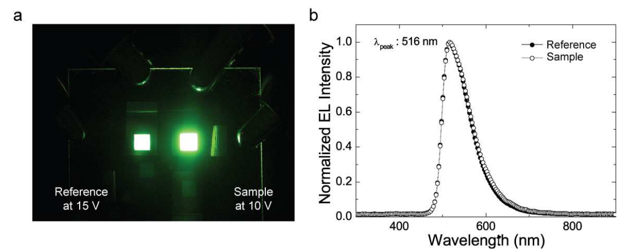
Fig. 3. (a) A photograph of the operating reference device (left) and sample device (right). The active area of each PHOLED is 3 × 3 mm². (b) The normalized EL spectra for the operating sample device (open circles) and reference device (closed circles). (Oh et al., 2007)
