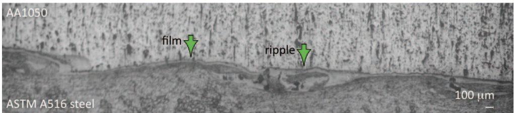
Fig. 7. Al/Fe interface (specimen ID 13).
