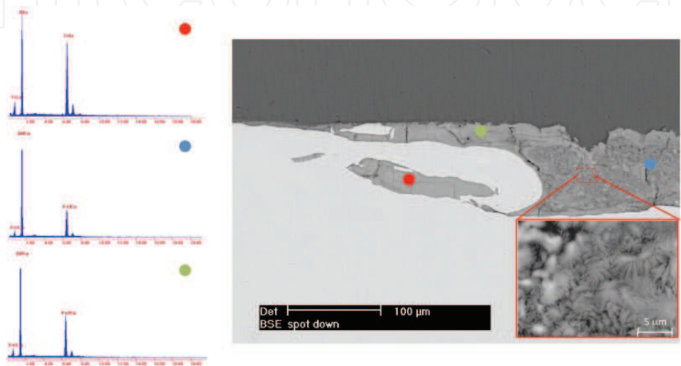
Fig. 4. SEM Observation.
