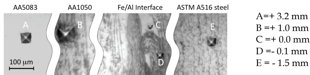
Fig. 8. Vickers indentations.
