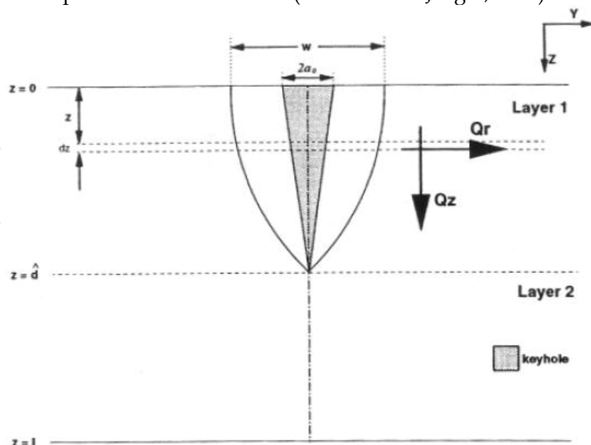
Fig. 3. Keyhole and the resulting weld profile, in which a work piece is sliced to many thin layers (Lankalapalli, Tu, and Gartner, 1996)
