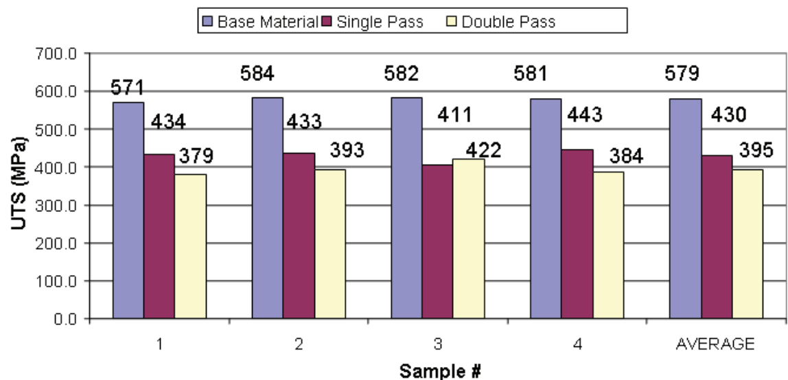
Fig. 15. Base AA 7075-T6 compared to single and double pass bead-on-plate welds
