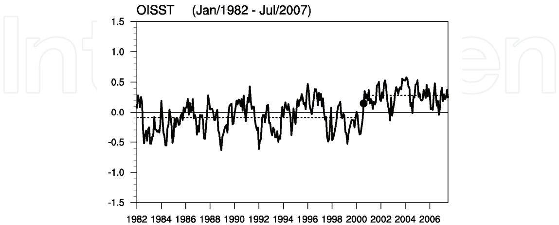
Fig. 8. Variation of monthly SST anomalies averaged over the area of 130°E-175°E and 5°S-5°N from January 1982 to July 2007. The short dashed lines are the means averaged over 1982-1999 (-0.1°C) and 2001-2006 (0.3°C) respectively. Adapted from Tu et al. (2009).
