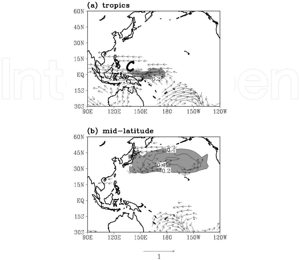
Fig. 7. SST anomalies (contour) and 850 hPa wind anomalies from the model simulations with the prescribed SST anomalies over (a) the equatorial region (130°E-175°E, 5°S-5°N) and (b) mid-latitudes (140°E-120°W, 25°N-45°N). Adapted from Tu et al. (2009).
