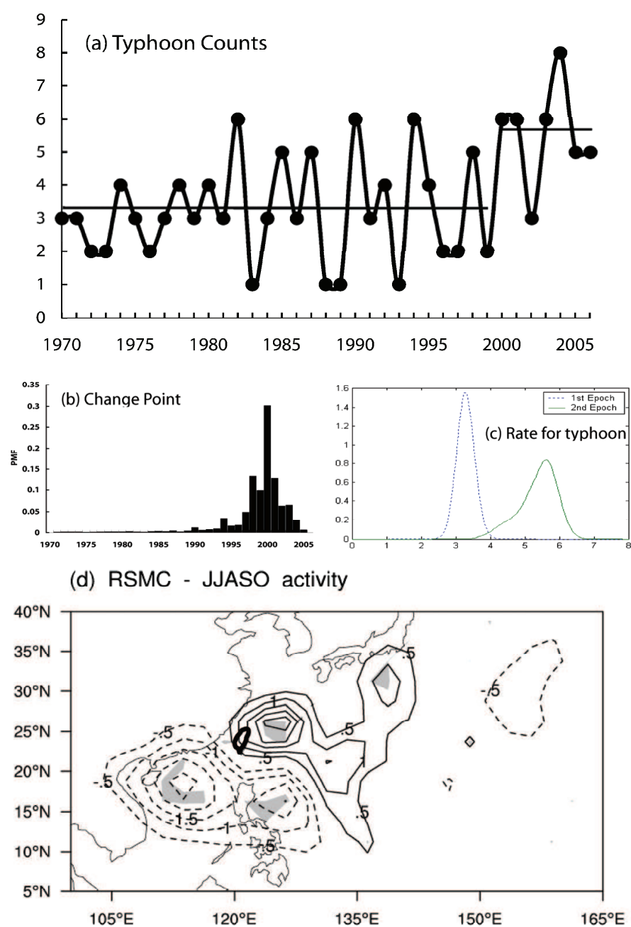
Fig. 3. (a) Time series of seasonal (JJASO) typhoon numbers passing the vicinity of Taiwan from 1970 to 2006 as compiled by the Central Weather Bureau. The vicinity was defined as 21°N-26°N and 119°E-125°E. (b) The conditional posterior probability mass function of change-points is plotted as a function of time. (c) Posterior density function of seasonal typhoon rate before (dashed line) and after (solid) the shift, with the change-point year being set in 2000. (d) June-October typhoon frequency differences for the period of 2000-2006 minus the period of 1970-1999 from the Regional Specialized Meteorological Center, Tokyo. The contour interval is 0.5; shading denotes that the difference between the mean of the two epochs is statistically significant at the 5% level. Adapted from Tu et al., (2009).
