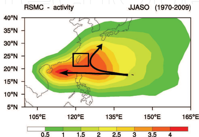
Fig. 1. June-October (JJASO) typhoon frequency climatology averaged over the period of 1970-2009. The contour interval is 0.5 per season (JJASO) per grid box (2.5°×2.5°). The bold arrows represent the majority of typhoon paths in the Western North Pacific-East Asian region. The box represents the area in the vicinity of Taiwan.
