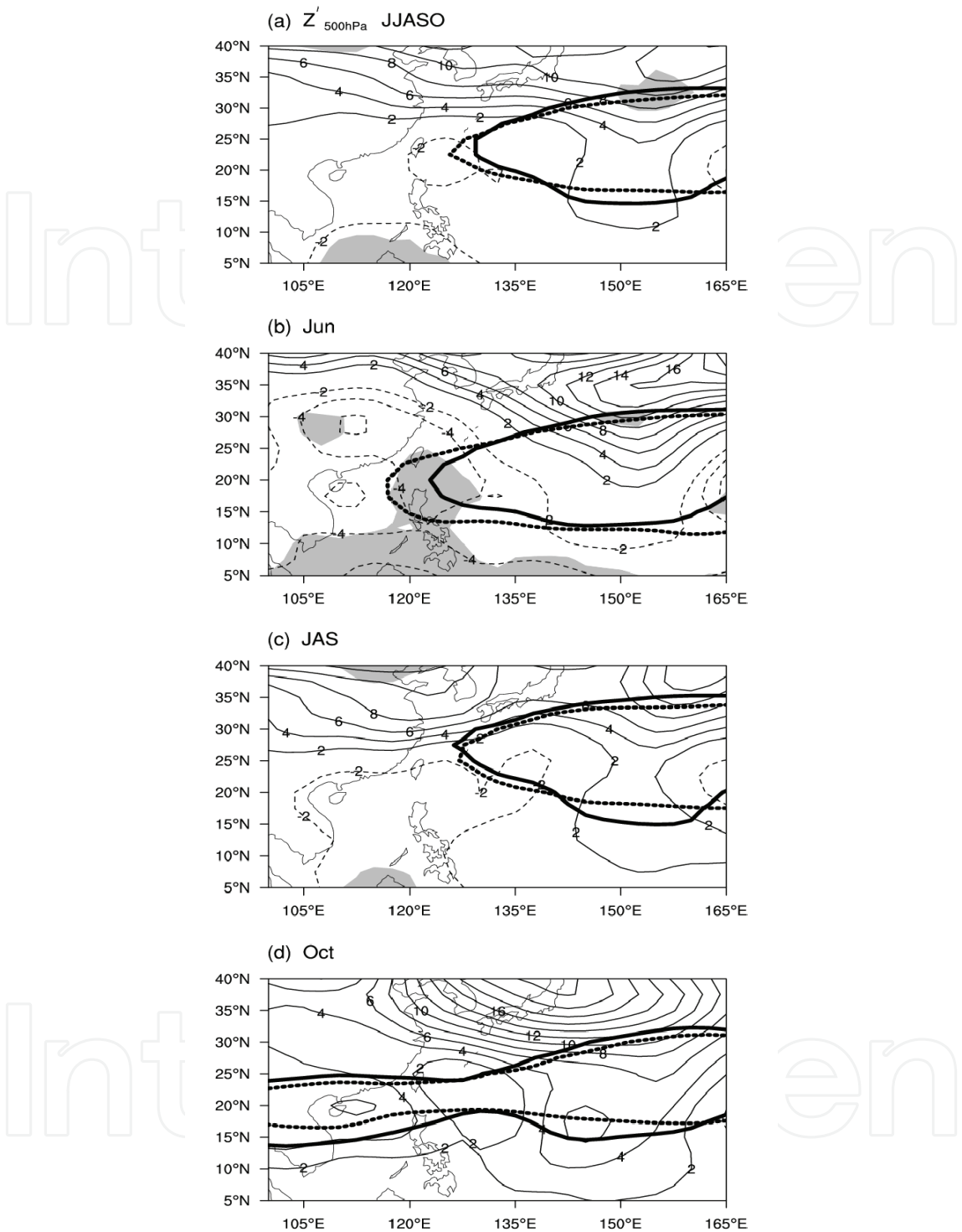
Fig. 5. The 5875 gpm contour of 500hPa geopotential height for the period of 1982-1999 (thick dotted line) and 2000-2006 (thick solid line) in (a) June-October (JJASO), (b) June, (c) July-September (JAS) and (d) October. The contours are the 500hPa geopotential height differences of the second minus first epoch, shaded by the 10% significance level. Adapted from Tu et al. (2009).
