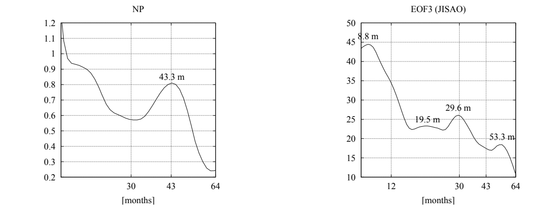
Fig. 16. Scale spectra of other climatic indices.
