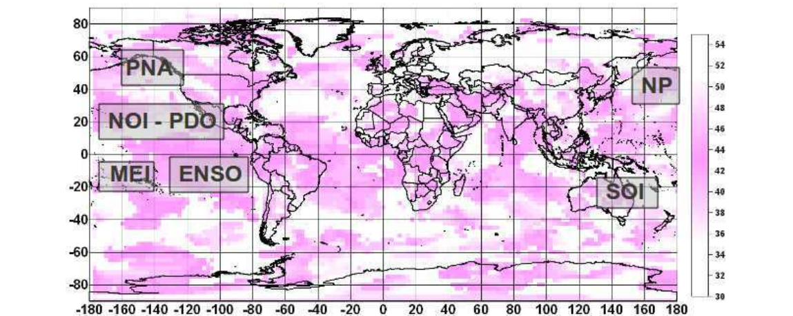
Fig. 12. NCEP/NCAR reanalysis data. The grid points where a cycle corresponding to c_2 has been detected are coloured.
