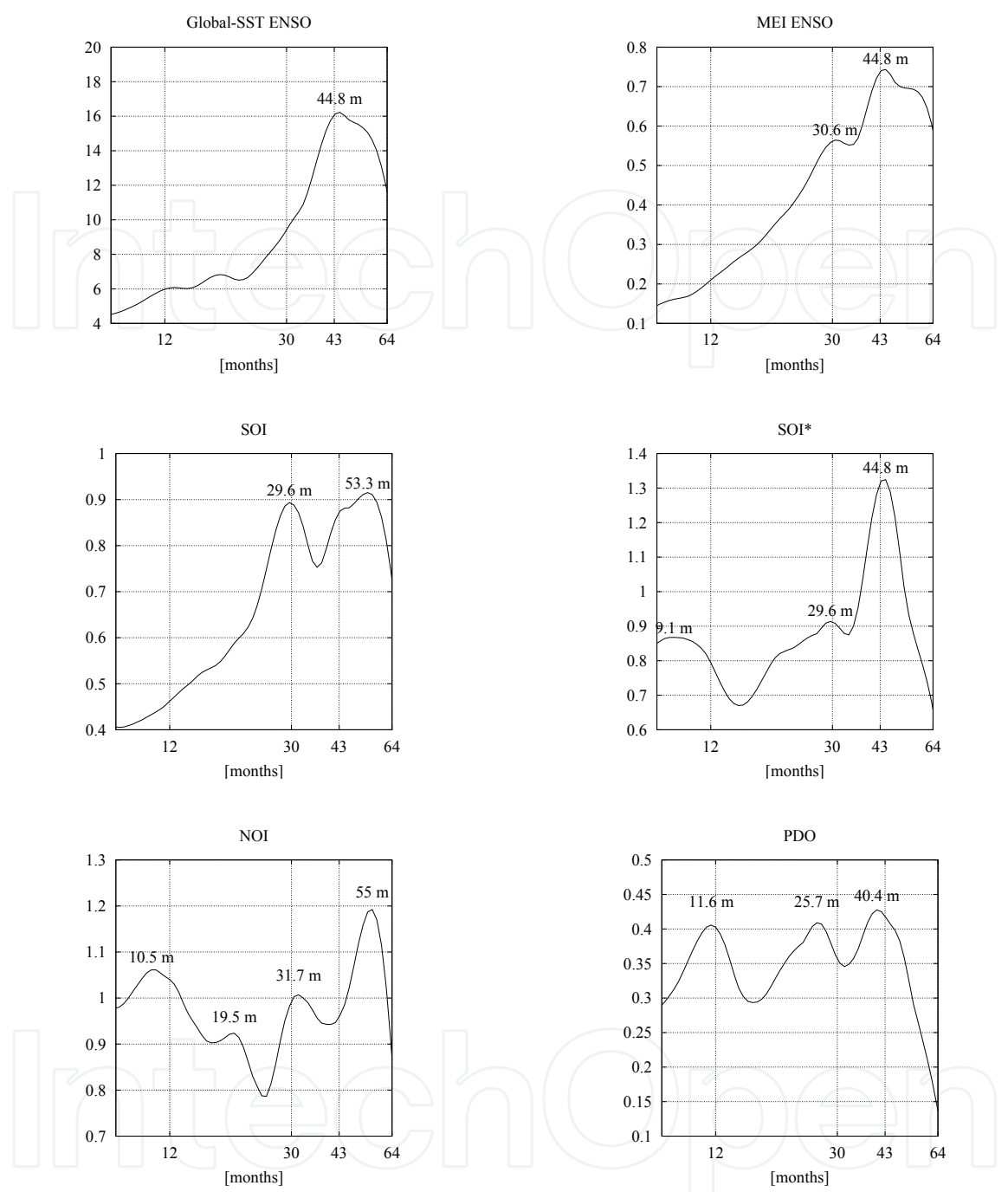
Fig. 14. Scale spectra of the climatic indices related to the Southern Oscillation.
