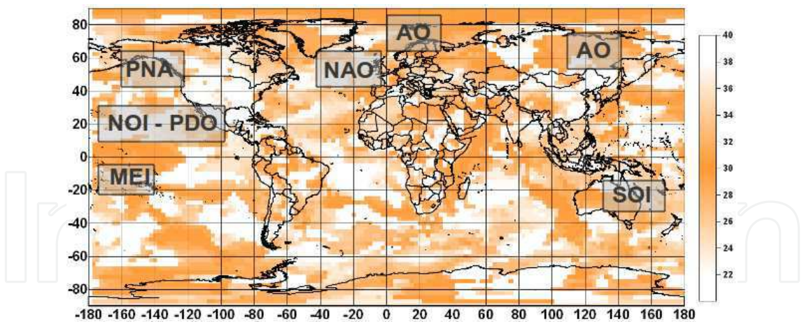
Fig. 11. NCEP/NCAR reanalysis data. The grid points where a cycle corresponding to c_1 has been detected are coloured.
