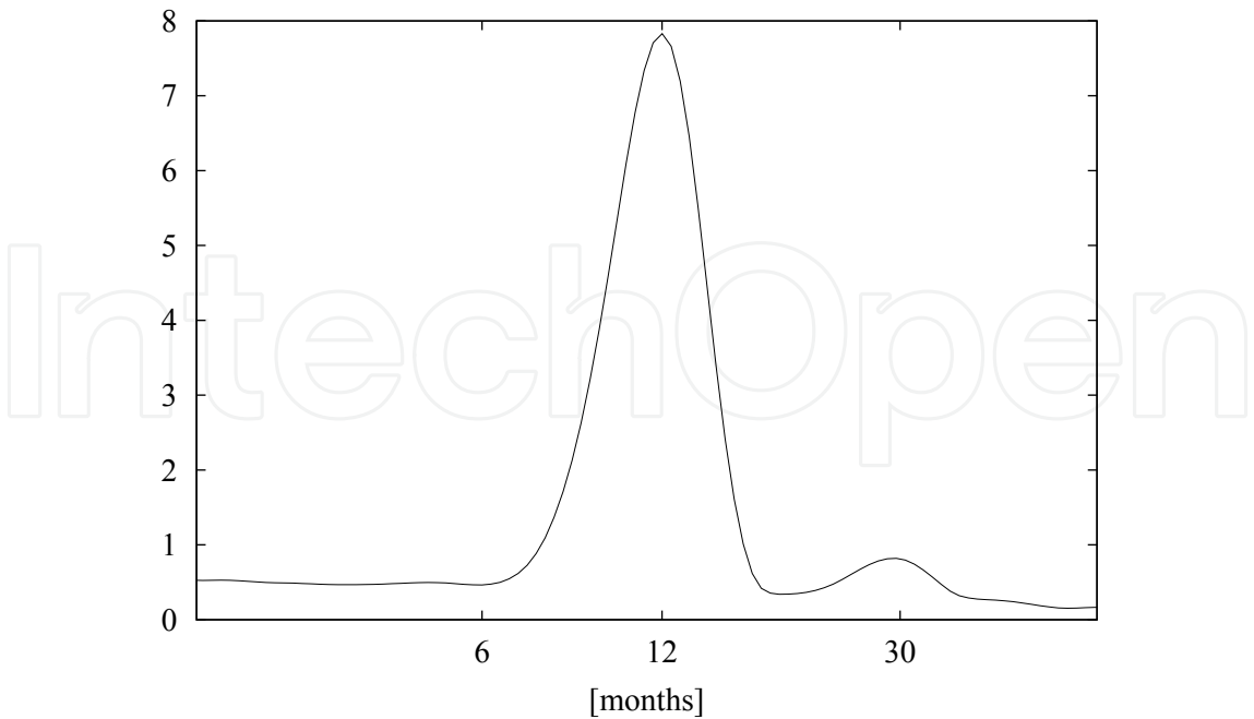
Fig. 3. The scale spectrum \Lambda of f . The abscissa (logarithmic scale) represent the months.
