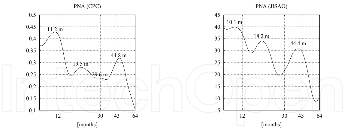
Fig. 15. Scale spectra of the PNA indices.
