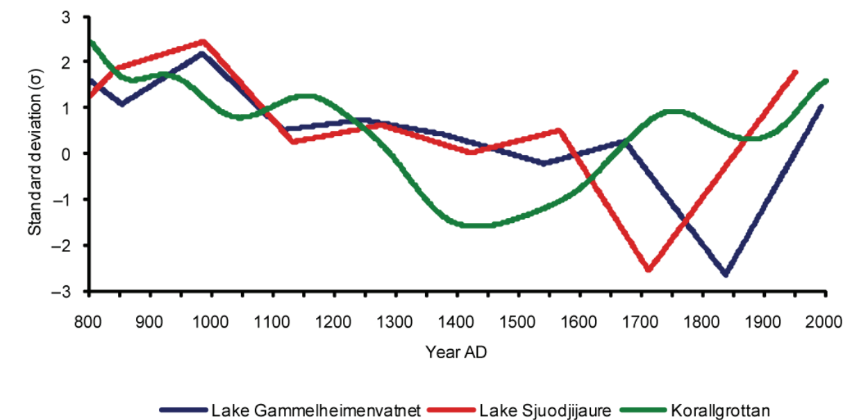
Fig. 4. Three normalised temperature records from Scandinavia shown relative to their AD 1000–1899 mean. The Korallgrottan record has been smoothed with a 100-year cubic spline filter.
