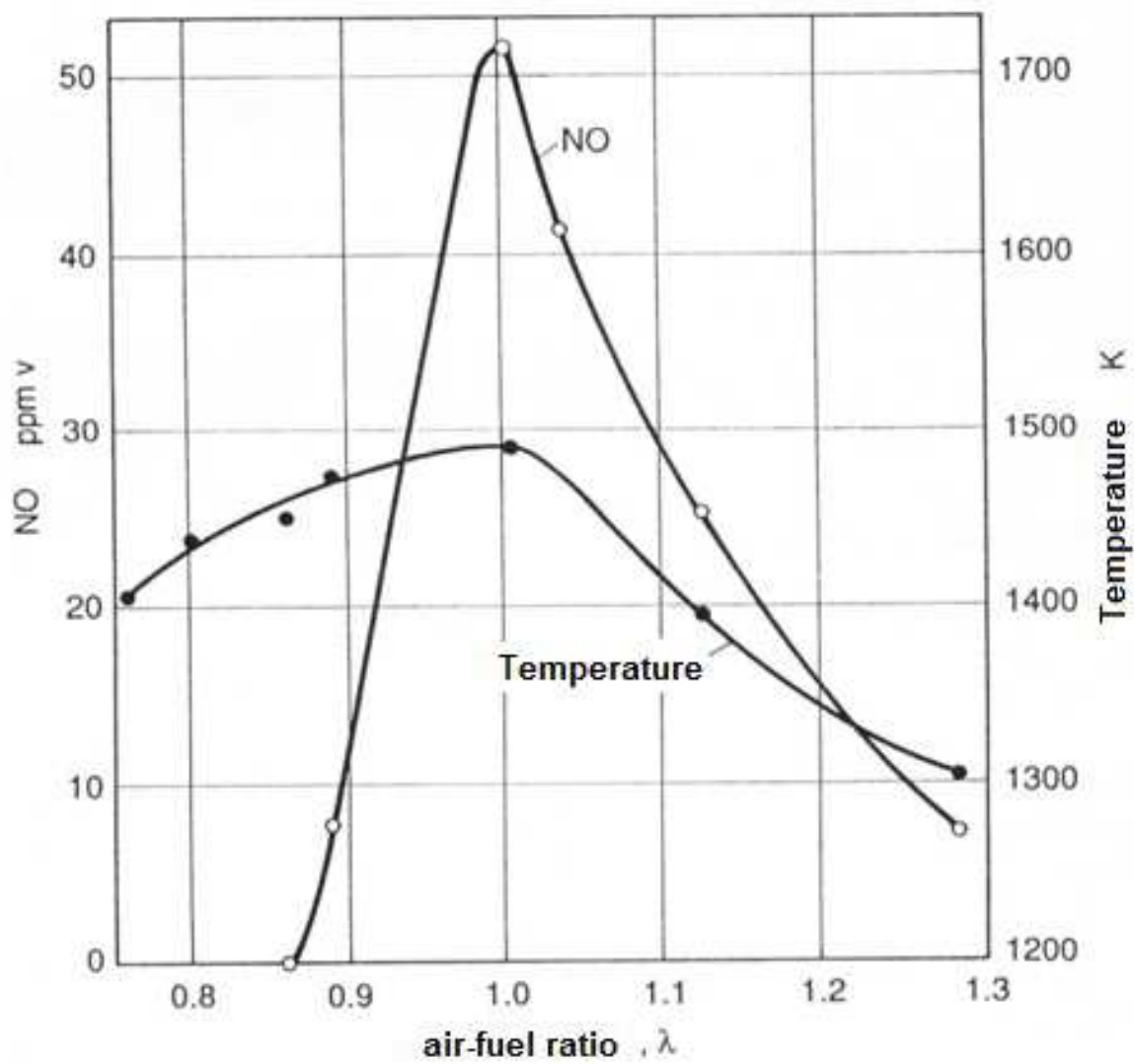
Fig. 7. Dependency between formed NO and combustion temperature and air-fuel ration (λ)
