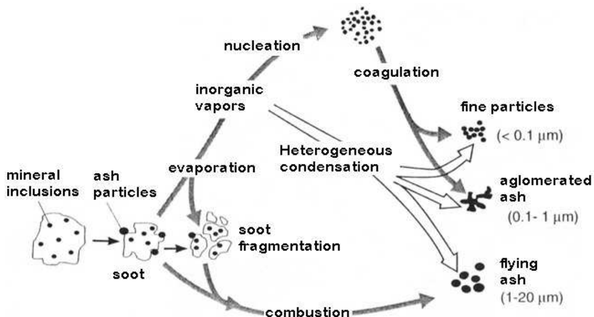
Fig. 15. Formation of particles in the combustion process of pulverized coal.
