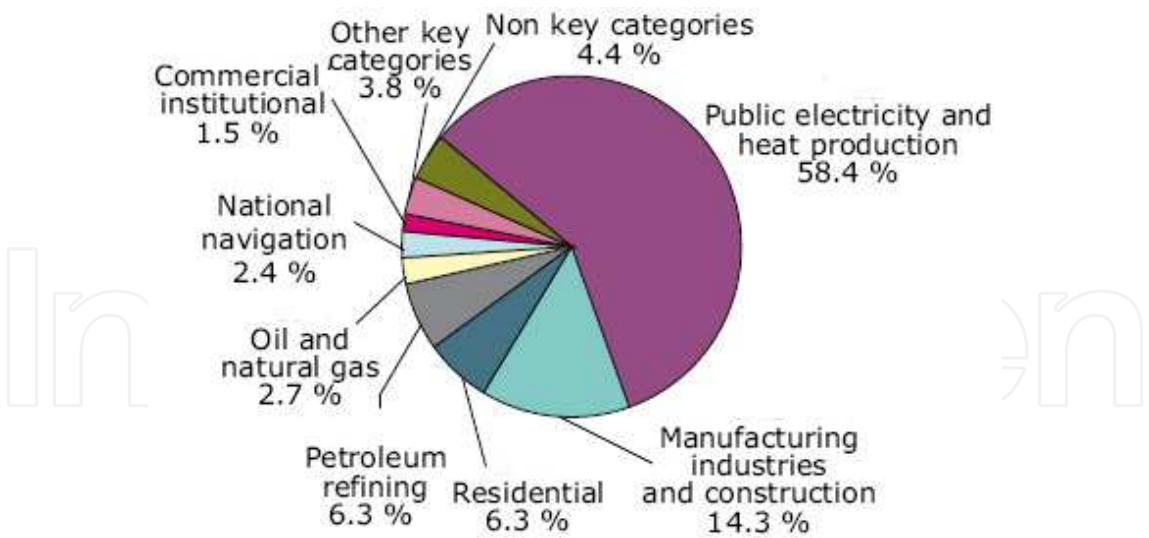
Fig. 9. EU-27 emission sources of sulphur oxides, 2006 (EEA, 2008).
