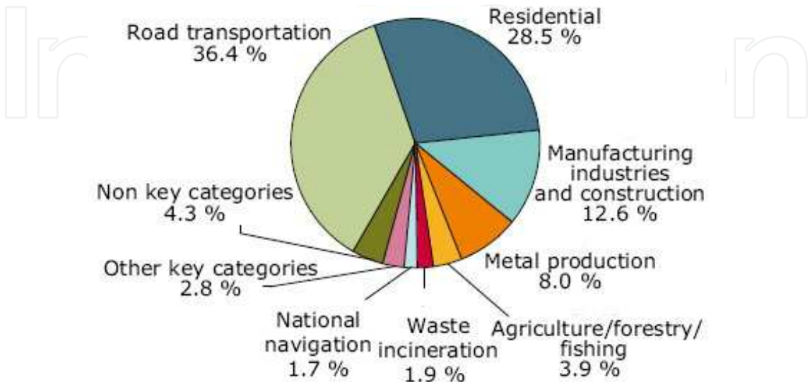
Fig. 3. EU-27 emission sources of carbon monoxide, 2006 (EEA, 2008).
