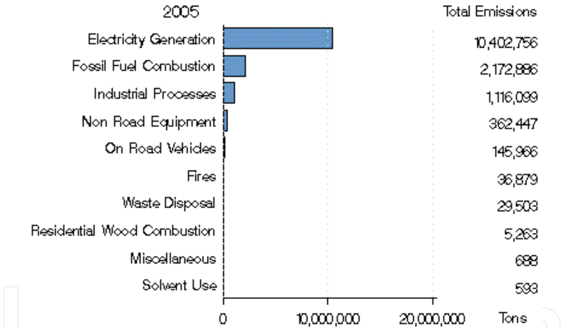
Fig. 10. USA emission sources of sulphur oxides, 2005 (US EPA, 2009).
