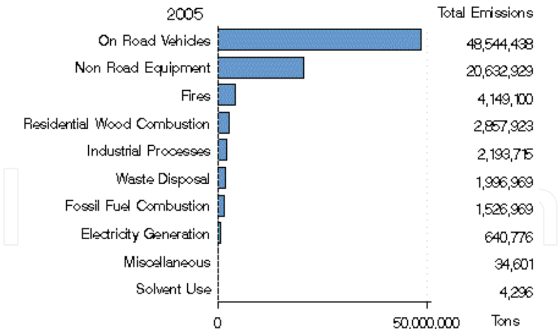
Fig. 4. USA emission sources of carbon monoxide, 2005 (US EPA, 2009).
