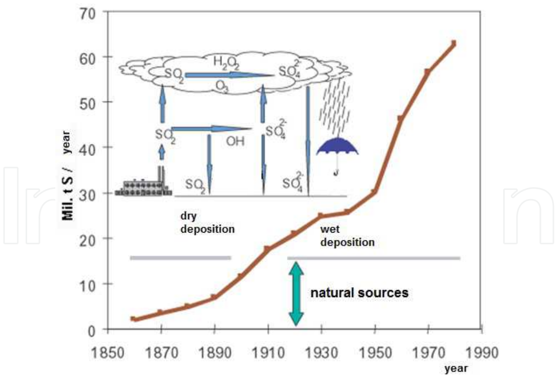
Fig. 11. SO 2 atmospheric reaction and historical emissions. (Popescu, 2009)
