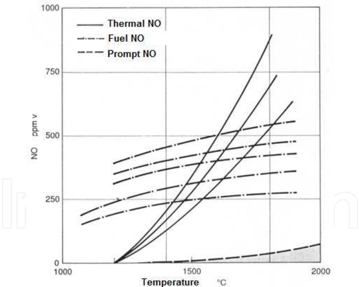
Fig. 8. Dependency between NO formation mechanisms and combustion temperature. Into exhaust gases the nitric oxides consists only in nitrogen oxide (NO). The oxidation of NO to NO 2 occurs partially in flue gases exhaust channels and in atmosphere, most important reactions are:
