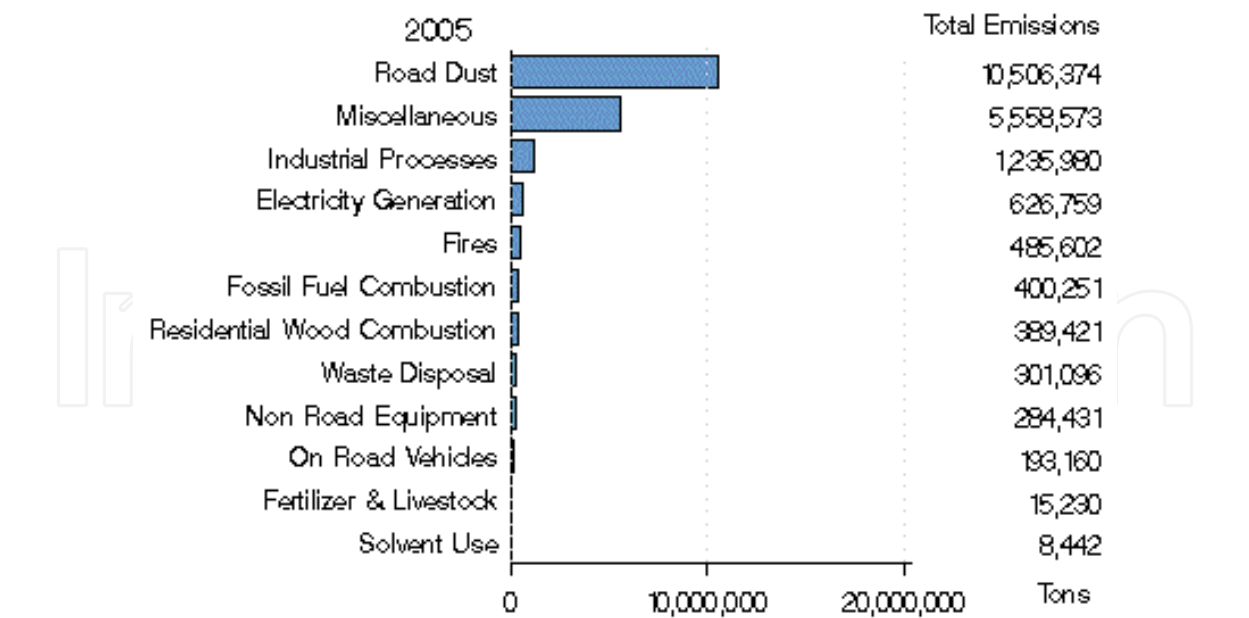
Fig. 13. USA emission sources of PM10, 2005 (US EPA, 2009).
