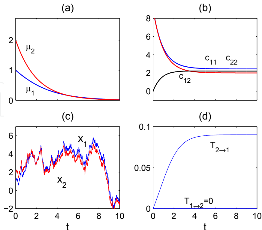
Fig. 2. A solution of (76) and the corresponding information transfers with the matrices \underline{\mathbf{A}} and \underline{\mathbf{B}} and initial condition as shown in the text. (a) \mu_1 and \mu_2 ; (b) c_{11} , c_{12} = c_{21} , c_{22} ; (c) a sample path starting from (1,2) ; (d) the computed information transfers T_{2 \rightarrow 1} (upper) and T_{1 \rightarrow 2} = 0 .
