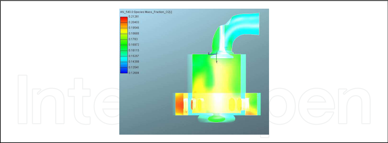
Fig. 9. 3D analysis for the calculation of the scavenging efficiency The 3D analysis also provides the definition of a proper heat release law, to be included in the 1D model, assuming injection in one shot. Figure 10 shows the 3D computed pressure cycle in comparison with the results of the 1D model. An idea of how the injection strategy affects combustion is also given. It is evident that a too advanced injection makes for a too much high pressure peak, which may be dangerous in terms of mechanical stresses, whereas a late injection makes for a low cycle area, hence a low power output and high fuel consumption.
