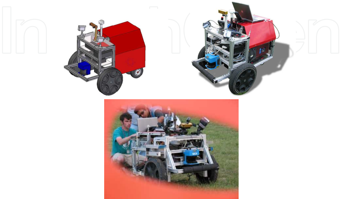
Fig. 8. Bearcat Cub intelligent vehicle designed for IGVC
