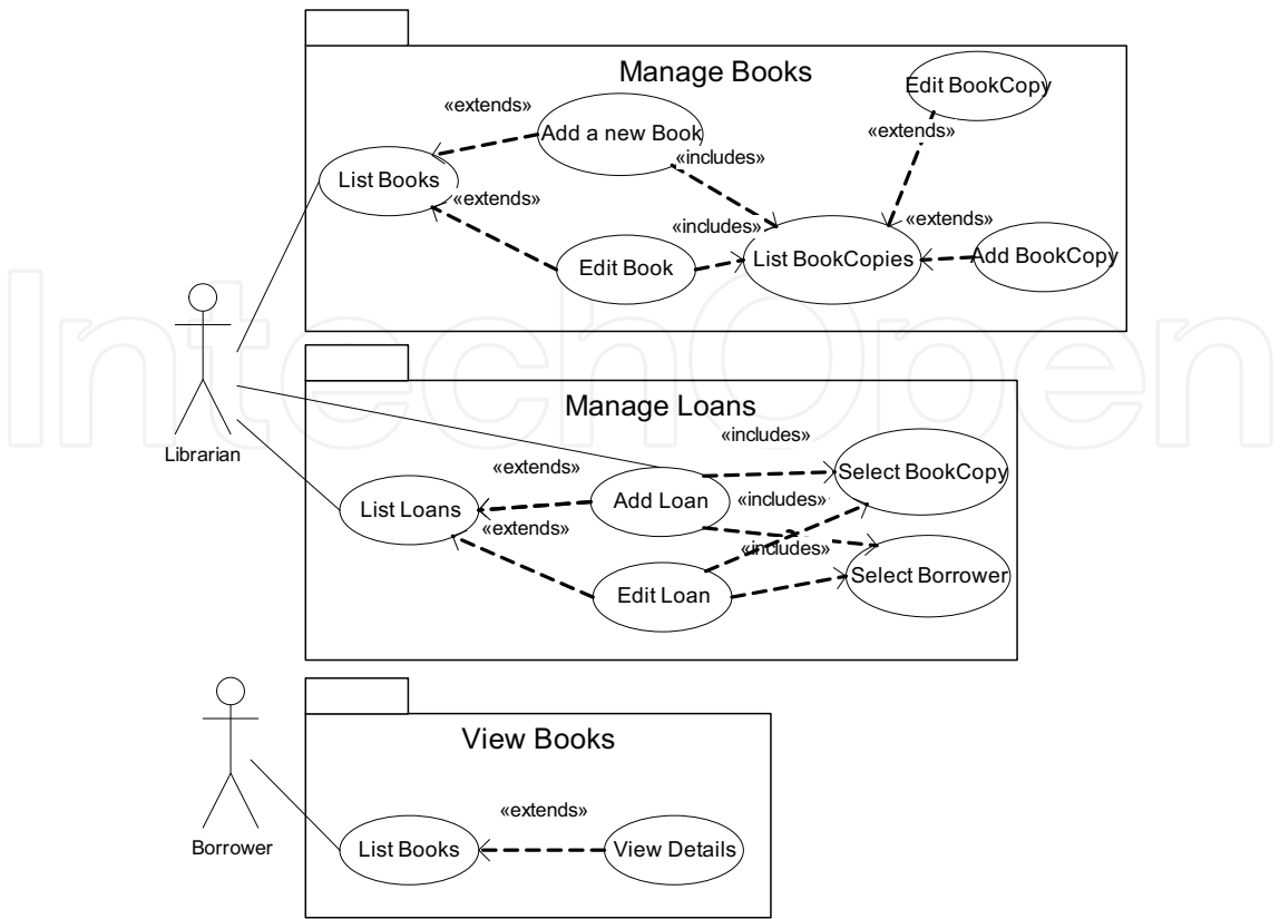
Fig. 7. Partial use case model (UCM) for the Library Management System.
