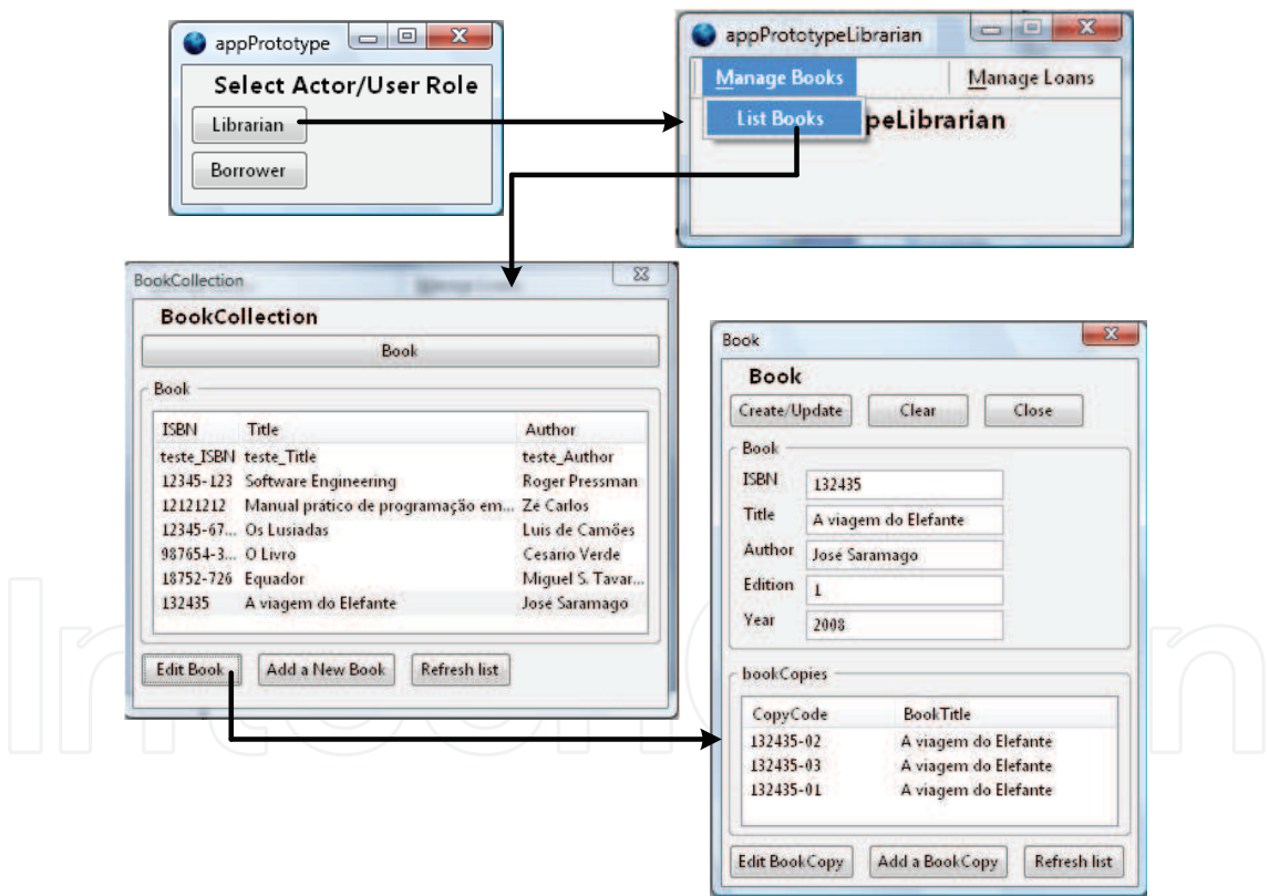
Fig. 8. Excerpt of the application prototype generated for a Librarian executing use cases List Books → Edit Book (that includes List BookCopies).
