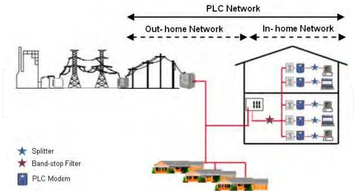
Fig. 16. In-home Network Model on Noisy Channels
