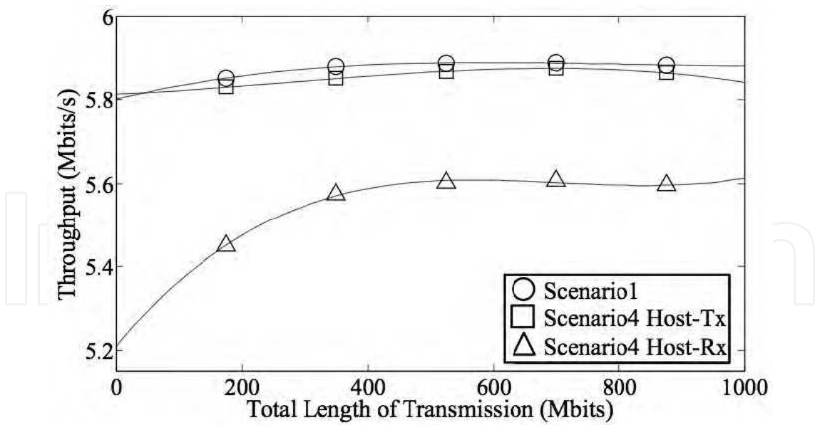
Fig. 8. Throughput for scenario 4
