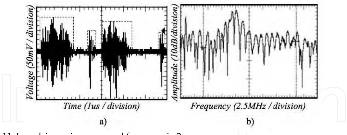
Fig. 11. Impulsive noise measured for scenario 2
