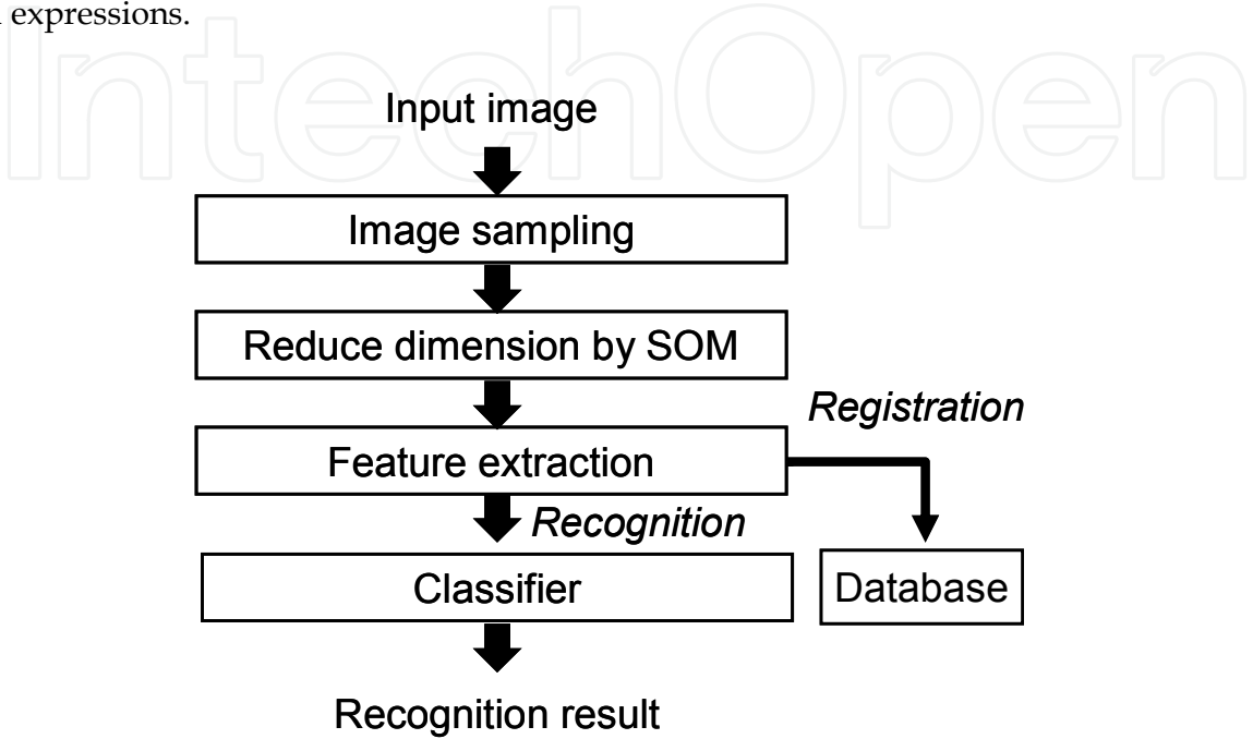
Fig. 2. General procedure of face recognition algorithm using Self-Organizing Map (SOM)
