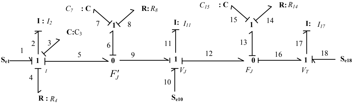
Fig. 5. Simplified bond graph model of the system
