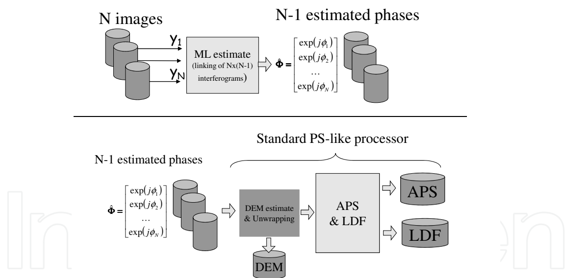
Fig. 4. Block diagram of the two step algorithm for estimating topography and subsidences.
