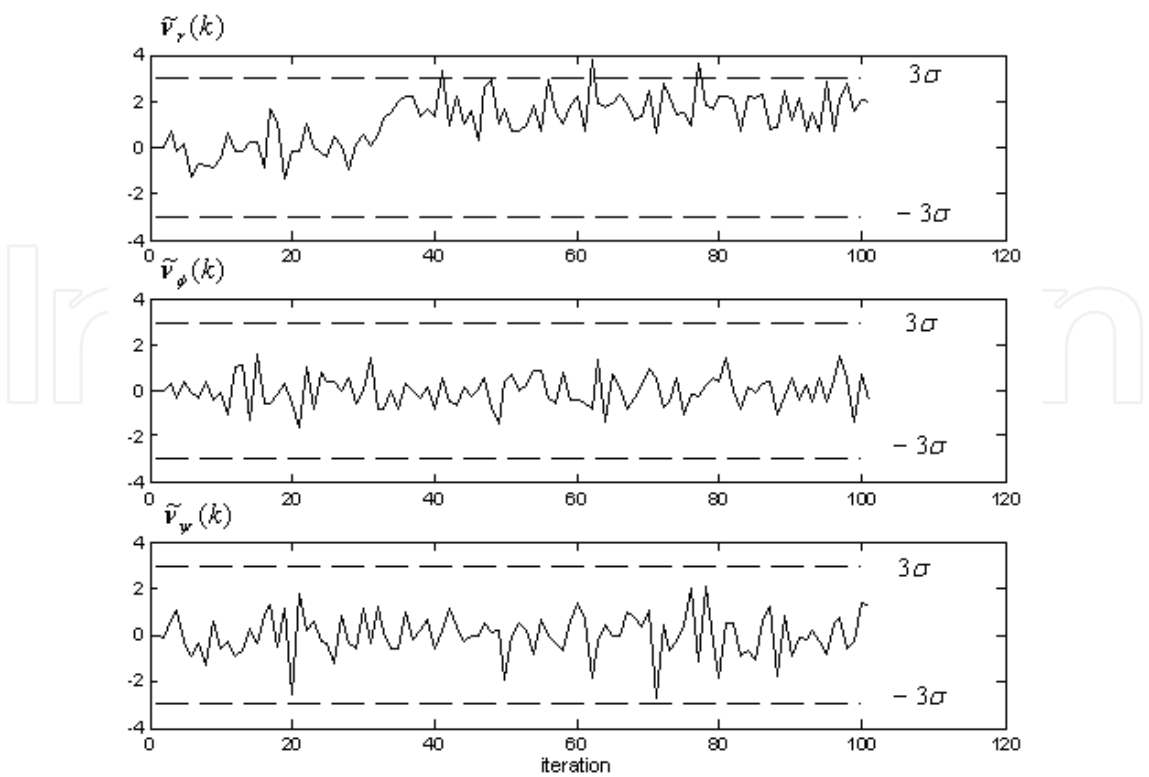
Fig. 12. Normalized Innovation Sequences \tilde{v}_r(k) , \tilde{v}_\phi(k) , \tilde{v}_\psi(k) in case of actuator motor failure
