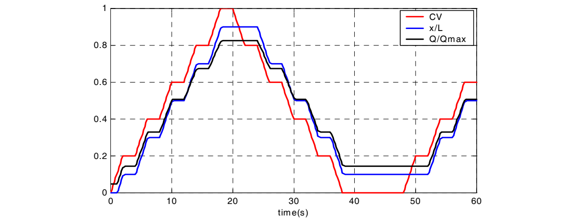
Fig. 7. Actuator works in “serious hysteresis” state
