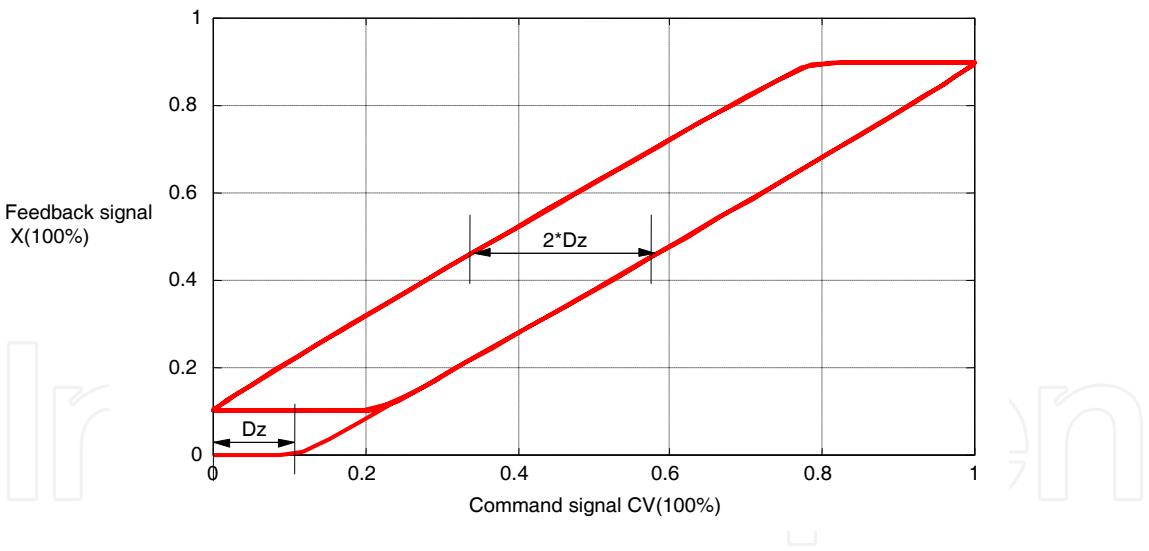
Fig. 15. X-Y graph with dead zone is D_z
