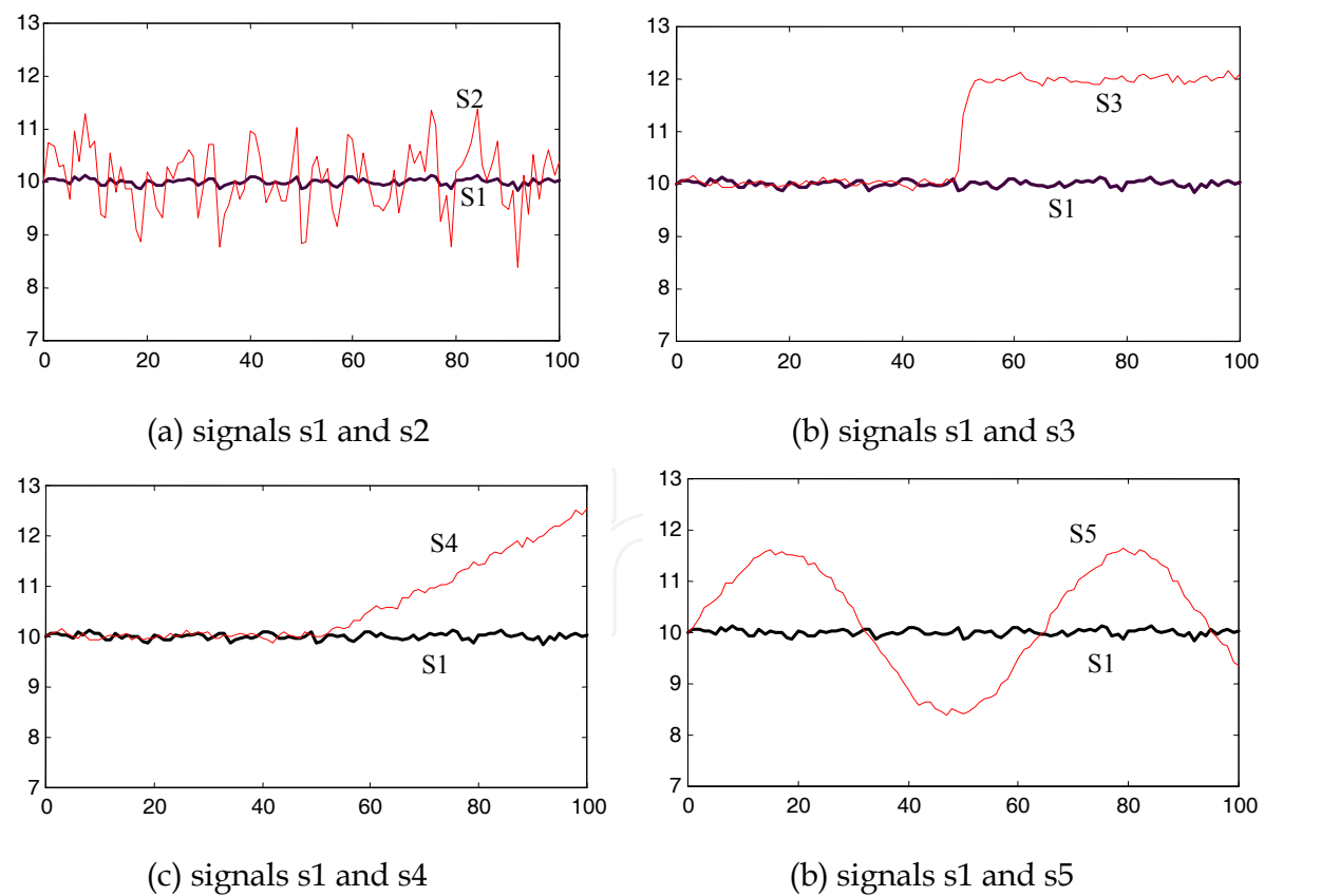
Fig. 17. The five typical signals for testing stable factor
