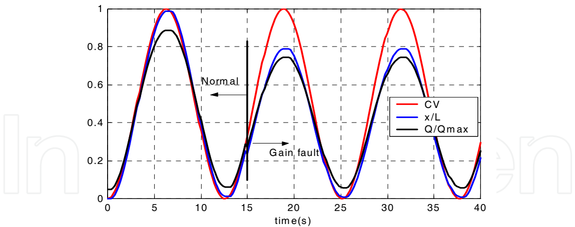
Fig. 6. Actuator works in “change of gain” state
