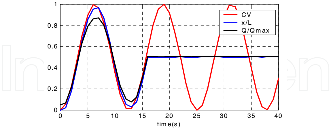
Fig. 8. Actuator works in “stuck” state
