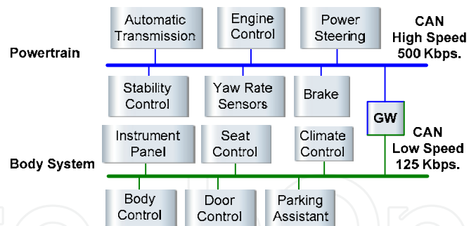
Fig. 4. CAN in automotive application.
