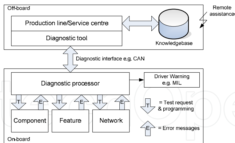
Fig. 7. Diagnostic scheme for in-vehicle electronic systems.
