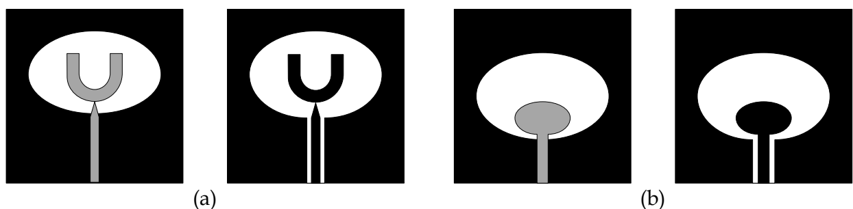
Fig. 17. The Microstrip-fed / CPW-fed UWB slot antennas
