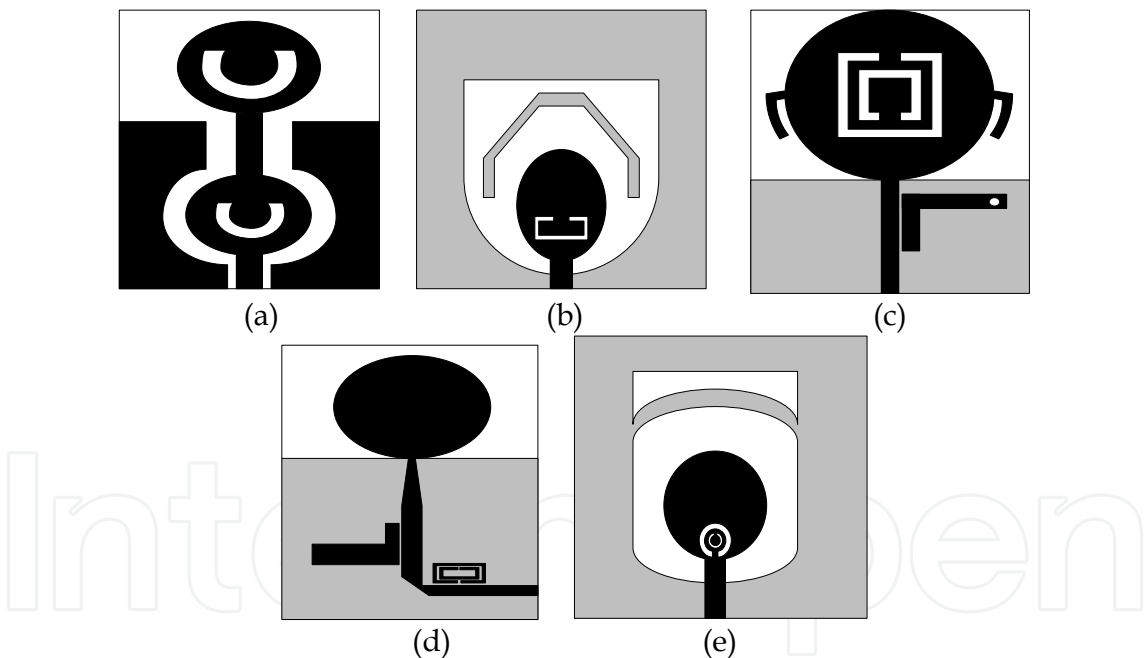
Fig. 31. Multiple band notched UWB antennas
