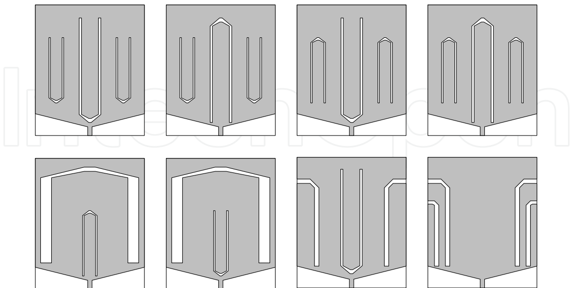
Fig. 30. The dual-band notched UWB antennas with slots
