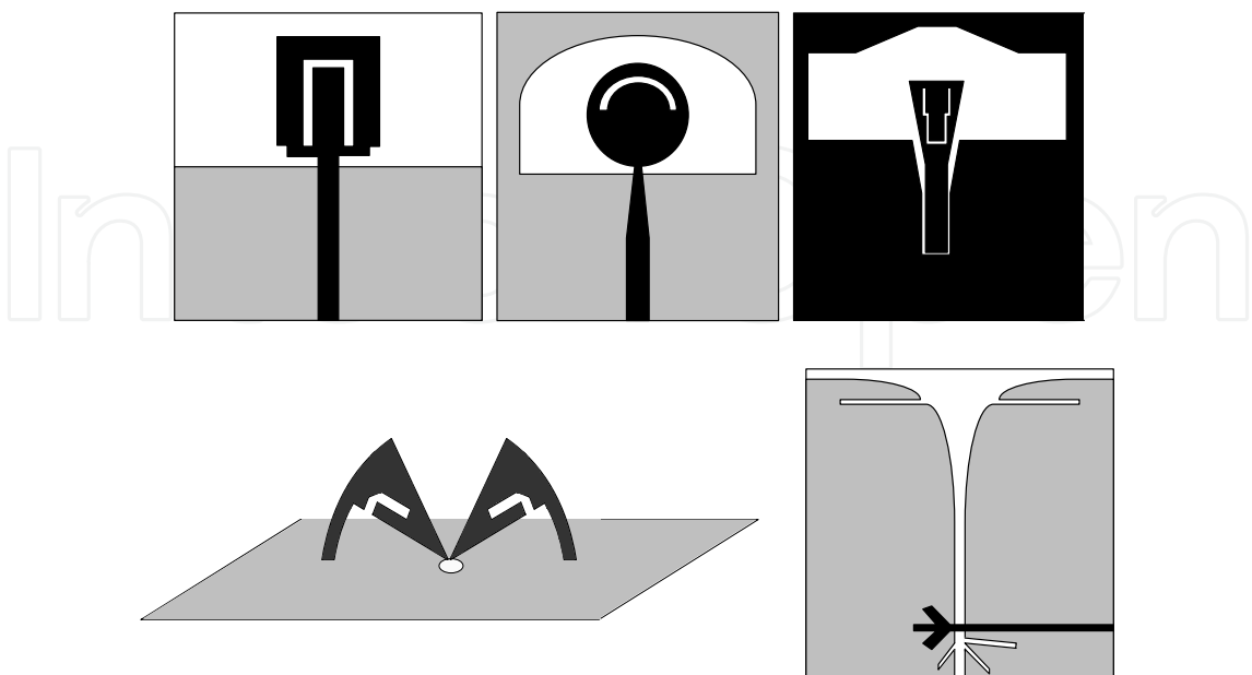
Fig. 20. The frequency notched UWB antennas using the slots on the radiating element
