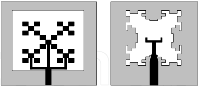
Fig. 26. The frequency notched UWB fractal slot antennas
