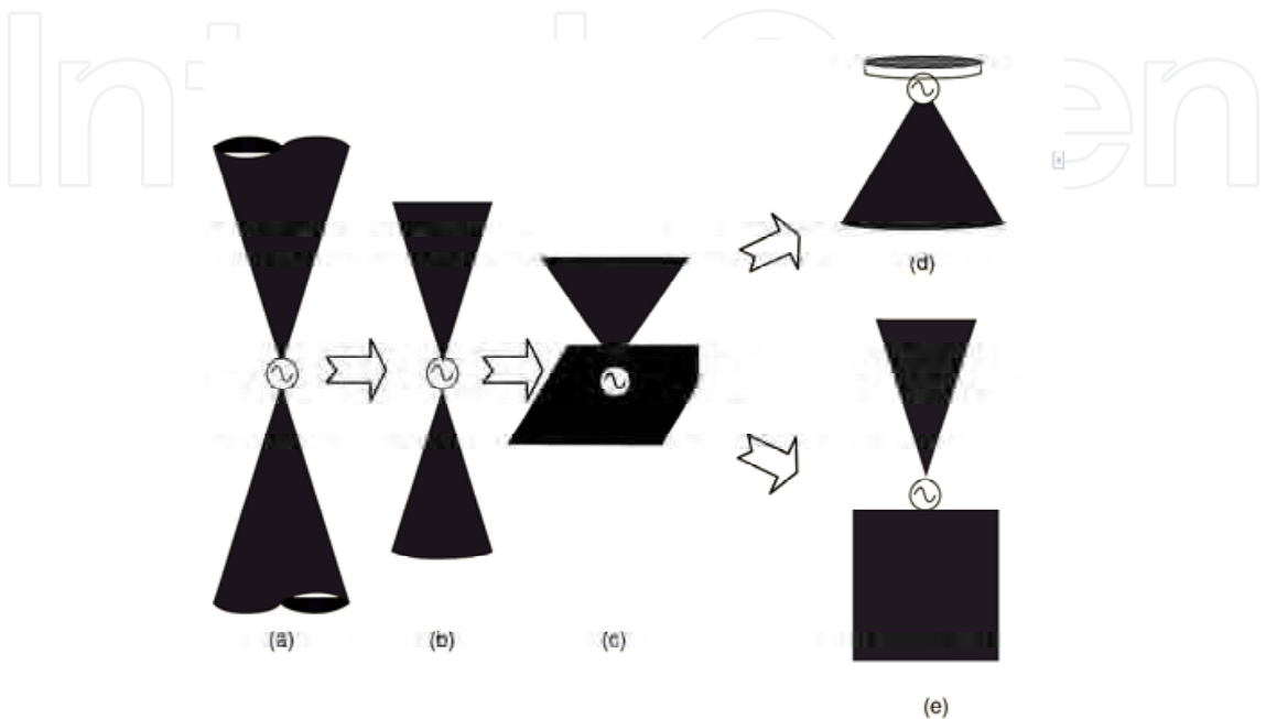
Fig. 7. Evolution processes from the conical antenna to disc cone antenna and planar monopole antenna
