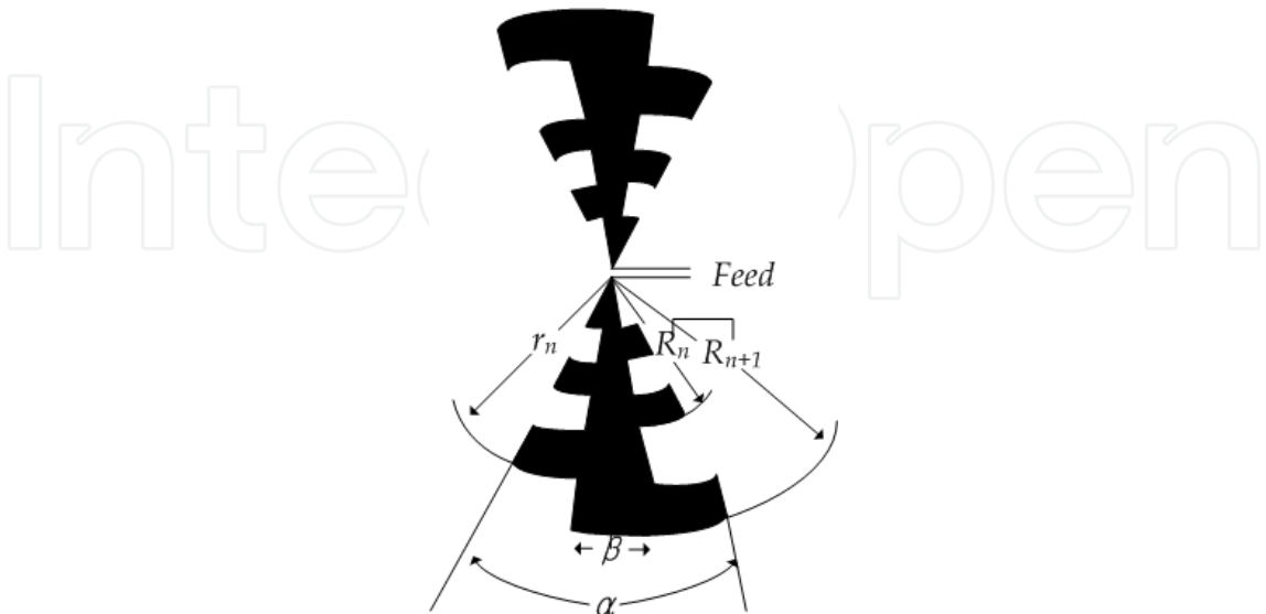
Fig. 5. The logarithmically periodic antenna structure
