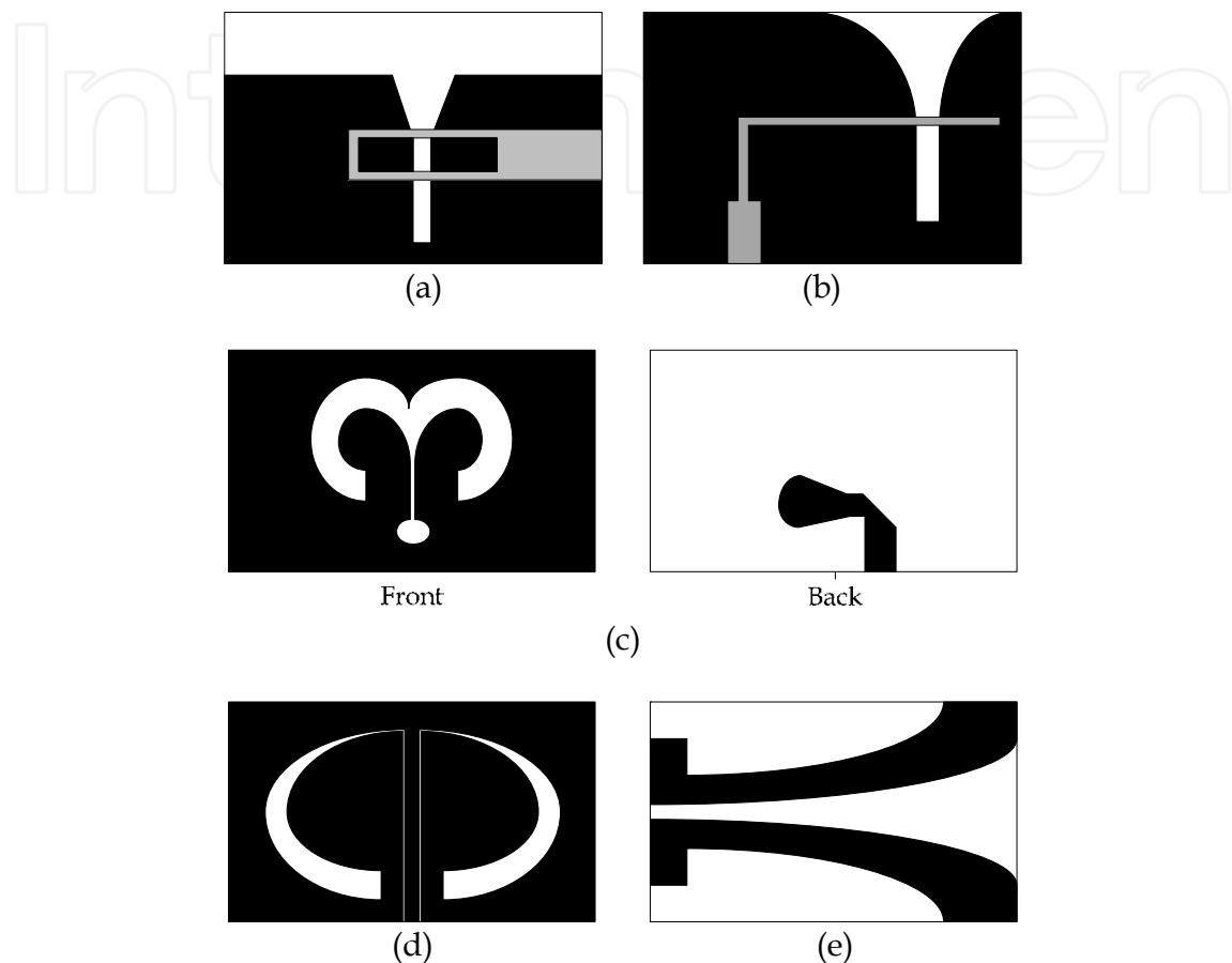
Fig. 18. The tapered slot antennas for UWB systems
