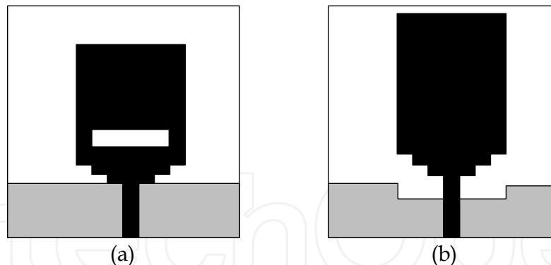
Fig. 11. The microstrip fed monopole antennas with rectangular patch
