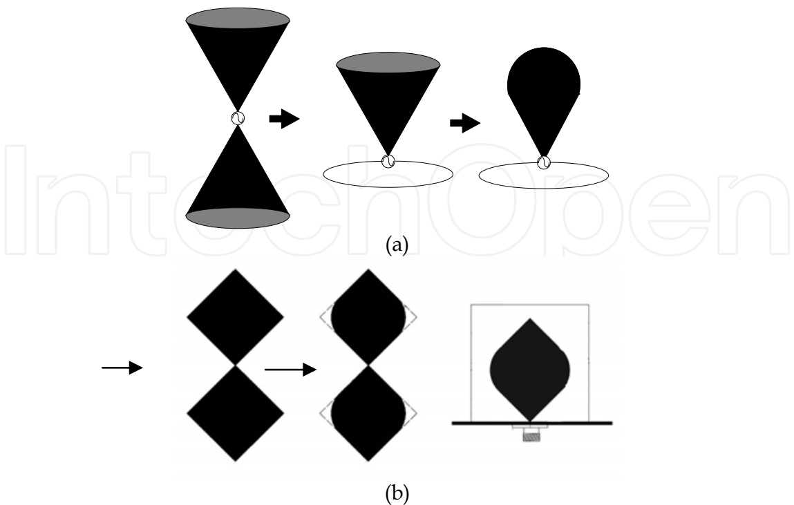
Fig. 8. The modified bowtie antenna structures
