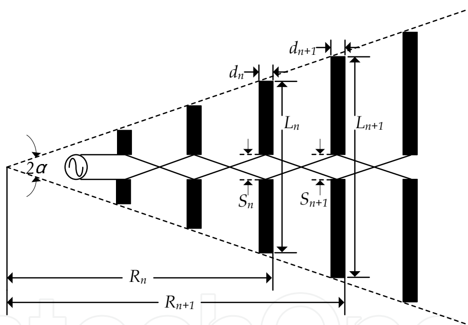
Fig. 6. The log-periodic dipole antenna geometry
