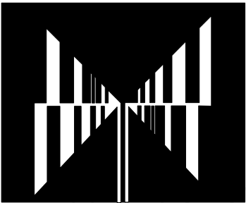
Fig. 25. The frequency notched log-periodic slot antenna
