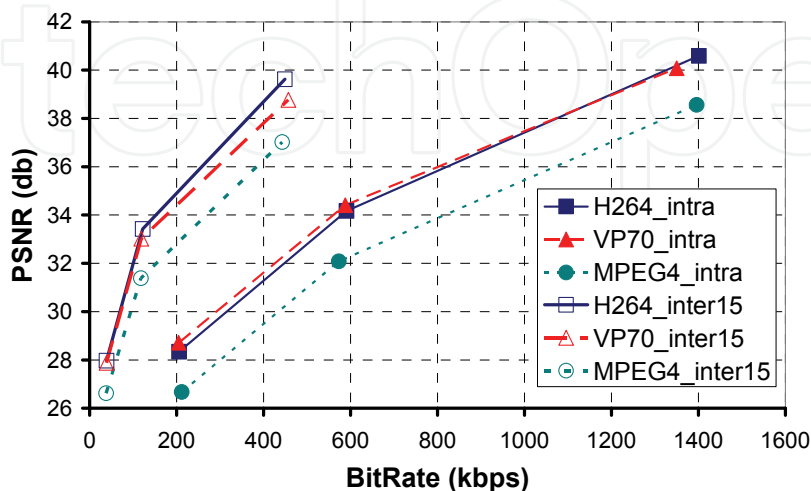
Fig. 5. R/D performance: objective PSNR quality comparison.
