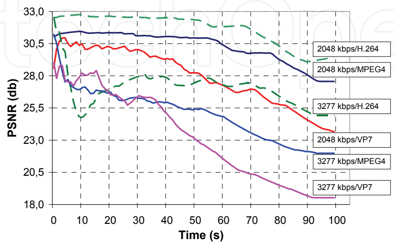
Fig. 14. Quality of reconstructed video with different codecs and traffic loads.
