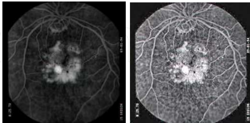
Fig. 5. Contrast enhancement by curvelets [Starck et al., 2003].
