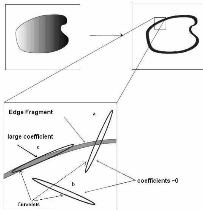
Fig. 3. Alignment of curvelets along curved edges [R]
