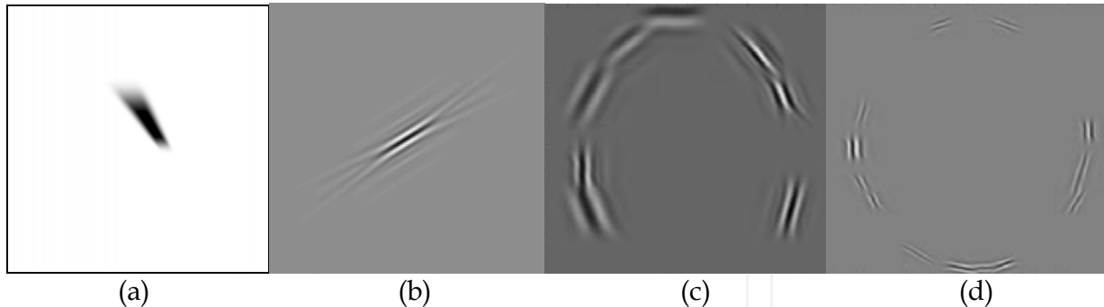
Fig. 2. (a) a real wedge in frequency domain, (b) corresponding curvelet in spatial domain [Candes et al. 2006], (c) curvelets aligned along a curve at a particular scale, (d) curvelets at a finer scale [Starck et al. 2002].
