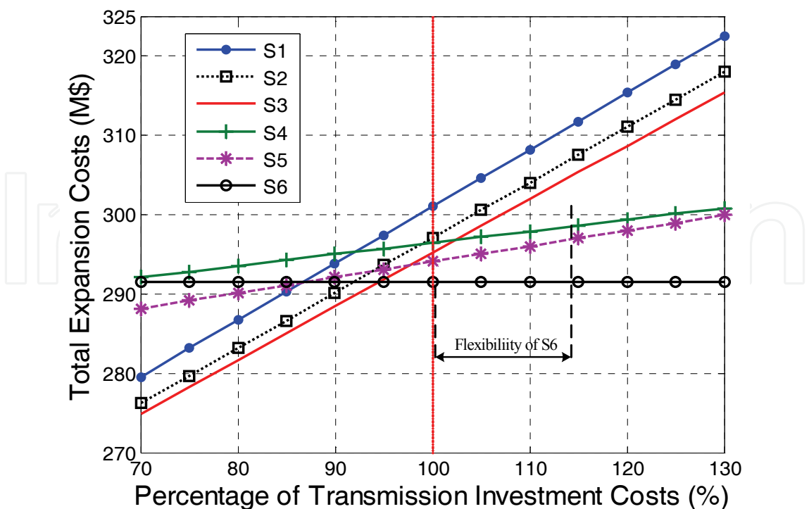
Fig. 11. Flexibility value for diverse transmission investment costs
