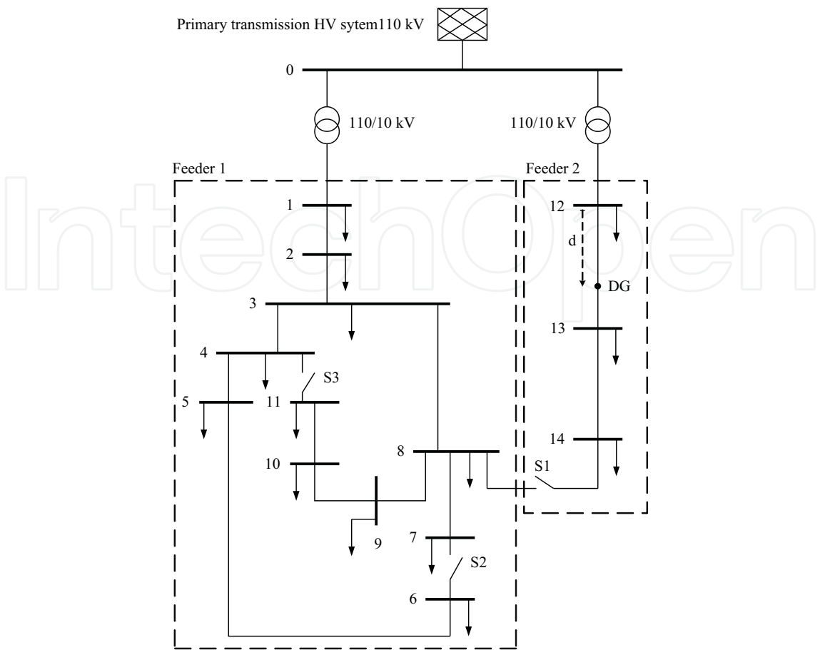
Fig. 10. Medium voltage benchmark network
