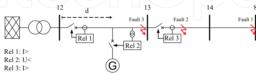
Fig. 15. Overview of all protection devices of Feeder 2
