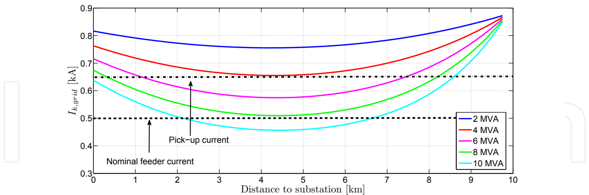
Fig. 11. Grid contribution as function of generator size and location
