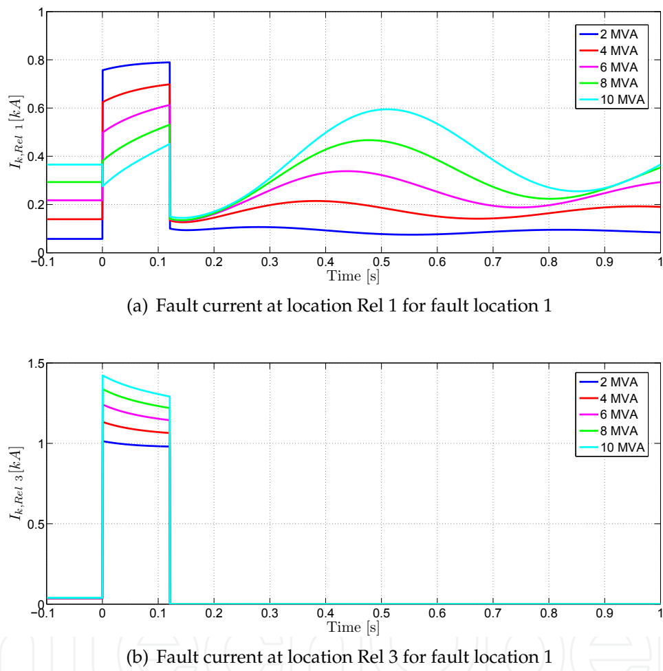
Fig. 17. Fault currents at relay location Rel 1 and Rel 3 for fault location 1
