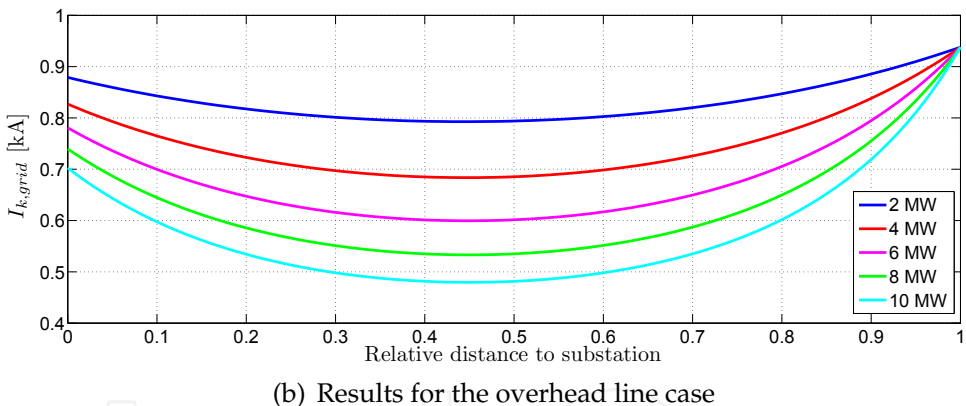
Fig. 5. Simulation results for the 3-bus test network
