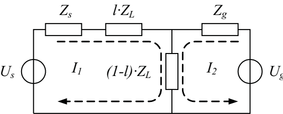
Fig. 2. Network equivalent of figure 1
