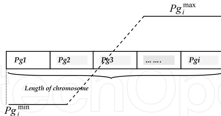
Fig. 5. Chromosome structure.
