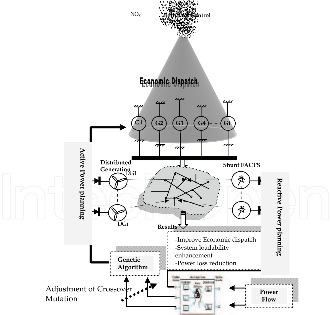
Fig. 1. Global strategy of OPF proposed with consideration of shunt FACTS and DG.
