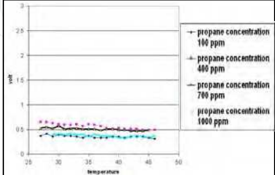
Fig. 24. Propane with TGS 3870 at R_L 7 k\Omega
