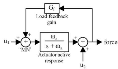
Fig. 9. Positive Feedback from Load Sensors.
