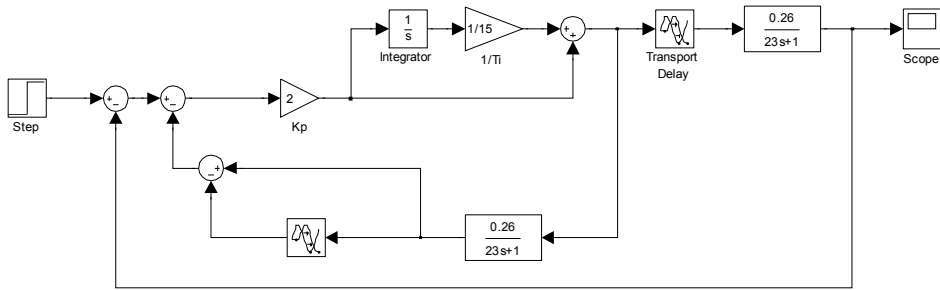
Figure 9. Smith Predictor in SIMULINK model.
