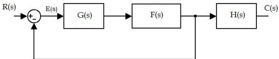
Figure 8. Equivalent system.
